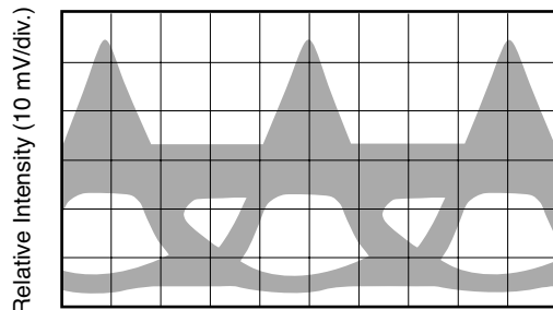
After 600 km (100 ps/div.)
