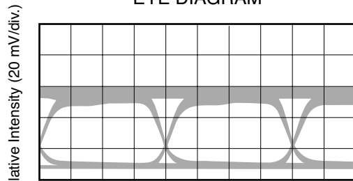
Back to Back (100 ps/div.)
