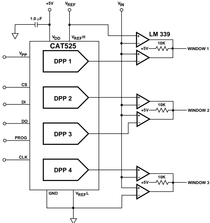
Overlapping Window Comparator
