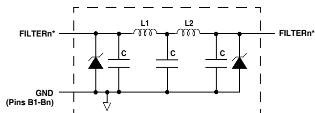
1 of n EMI Filtering + ESD Channels (n = 6 for CM1450-06, 8 for CM1450-08)
