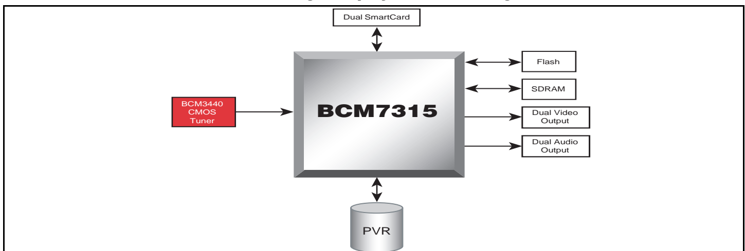
BCM7315 Single-Chip System Block Diagram
