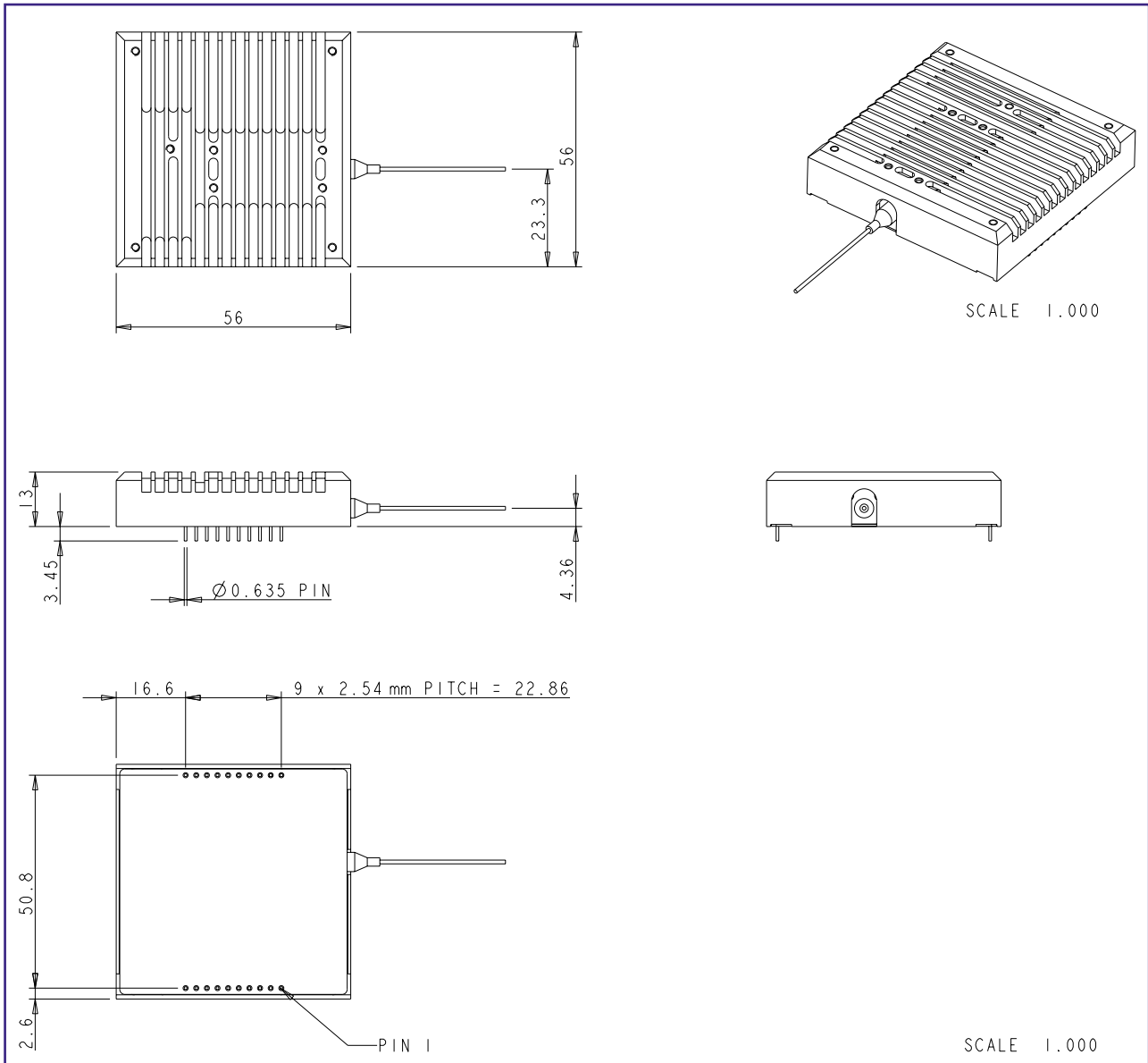
Figure 2: Mechanical outline
