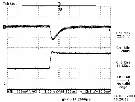
50% to 100% load Transient at V_{in}=5\text{ V} , V_o=2.5\text{ V}
