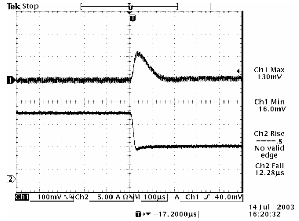
100% to 50% load Transient at V_{in}=5\text{ V} , V_o=1.8\text{ V}
