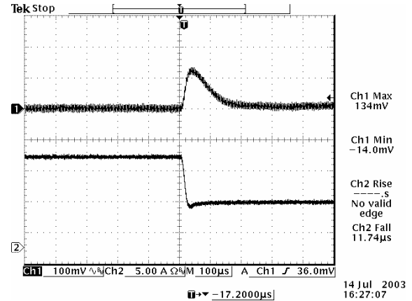
100% to 50% load Transient at V_{in}=5\text{ V} , V_o=2.5\text{ V}
