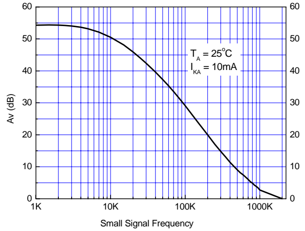
Figure 7. Voltage Reference Small Signal Voltage Gain vs. Frequency
