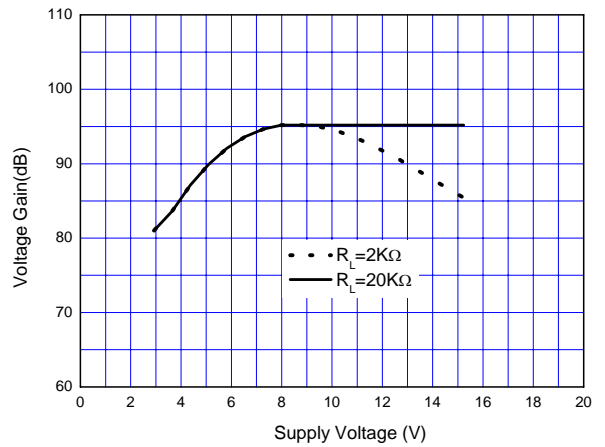
Figure 9. Op Amp Voltage Gain
