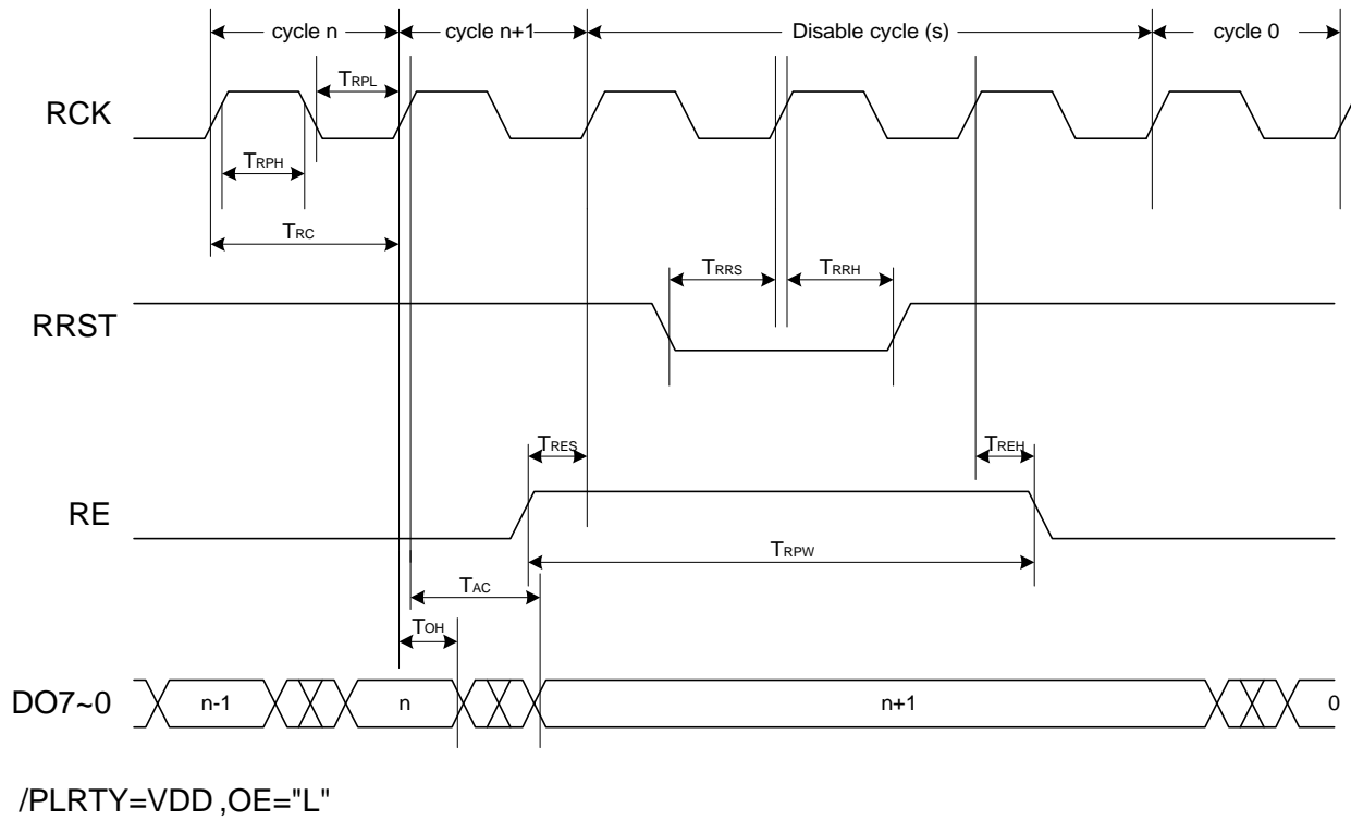
Read Cycle Timing (RE, RRST)
