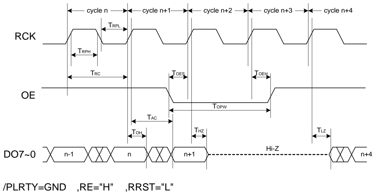
Read Cycle Timing (Output Enable)
