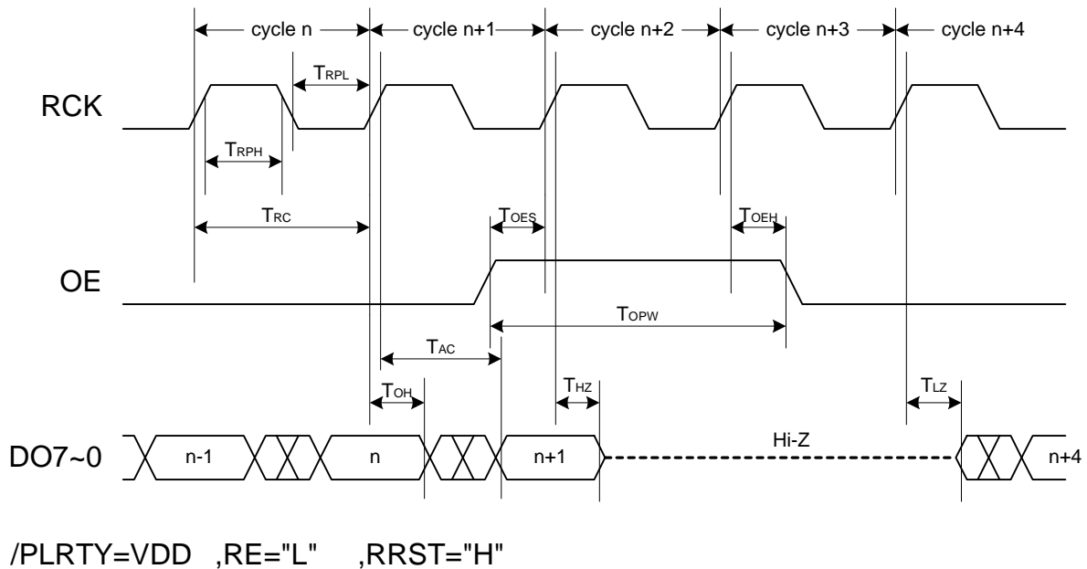
Read Cycle Timing (Output Enable)
