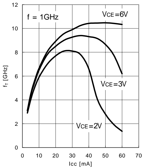
Transition Frequency : f_T vs. I_{CC}
