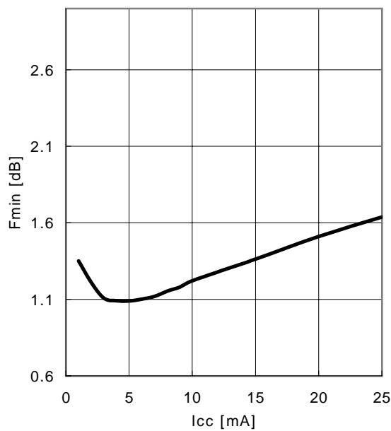
F_{min} vs. I_{cc} V_{CE} = 8\text{V} , I_{cc} = \text{parameter} , Z_s = Z_{spot}
