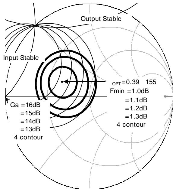
Noise Figure Contours & Constant Gain f = 1\text{GHz} , V_{CE} = 8\text{V} , I_{cc} = 5\text{mA}
