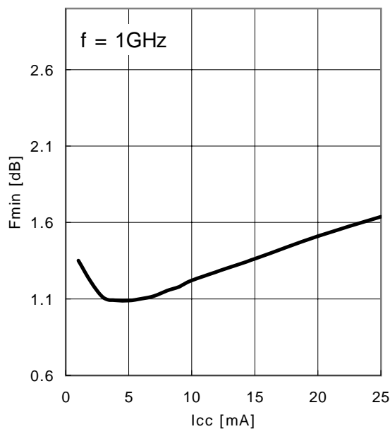
F_{min} vs. I_{cc} V_{CE} = 8\text{V} , I_{cc} = \text{parameter} , Z_s = Z_{opt}
