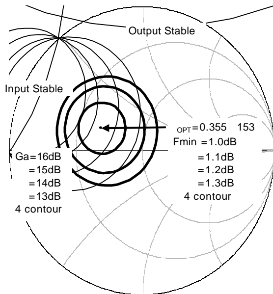
Noise Figure Contours & Constant Gain f = 1\text{GHz} , V_{CE} = 8\text{V} , I_{cc} = 5\text{mA}
