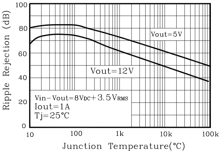
Fig. 5 Ripple Rejection
