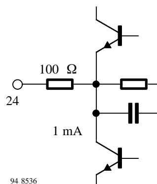
Figure 20. Intermodulation output (Pin 24)
