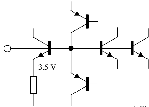
Figure 15. Internal reference voltage (Pin 17)
