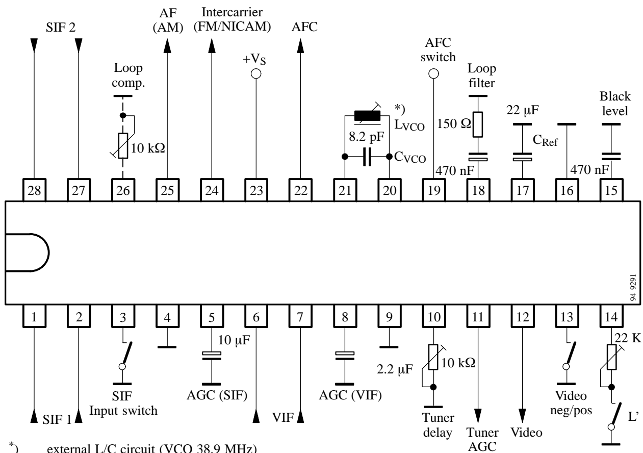
Figure 3. Test circuit
