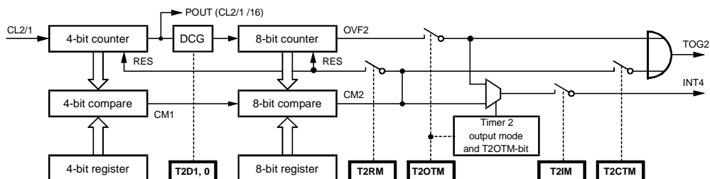
Figure 37. 12-bit Compare Counter
