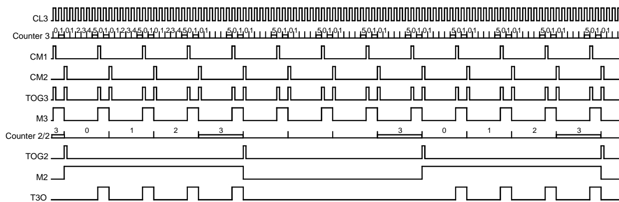
Figure 88. Burst Modulation 1
