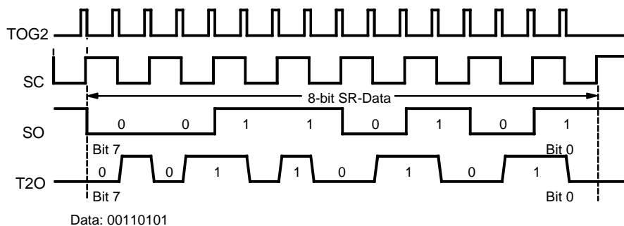
Figure 47. Manchester Modulation
