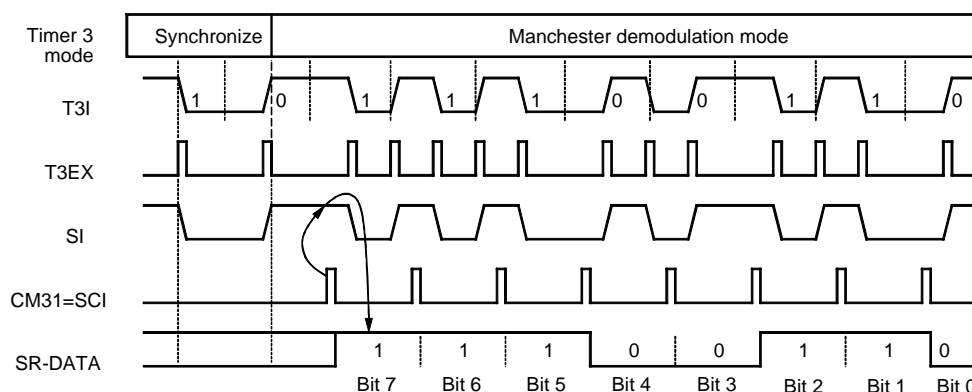
Figure 83. Manchester Demodulation
