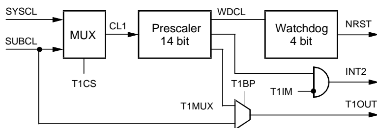
Figure 34. Timer 1 Module
