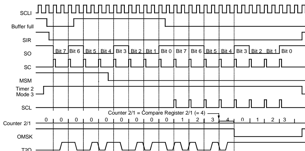
Figure 78. Manchester Modulation 2
