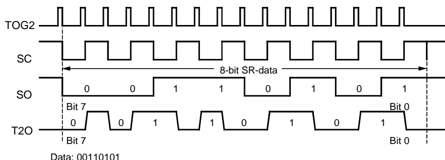
Figure 77. Manchester Modulation 1
