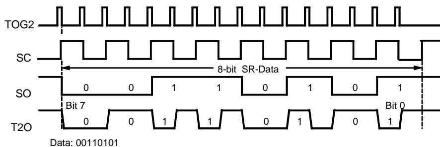
Figure 46. Biphase Modulation
