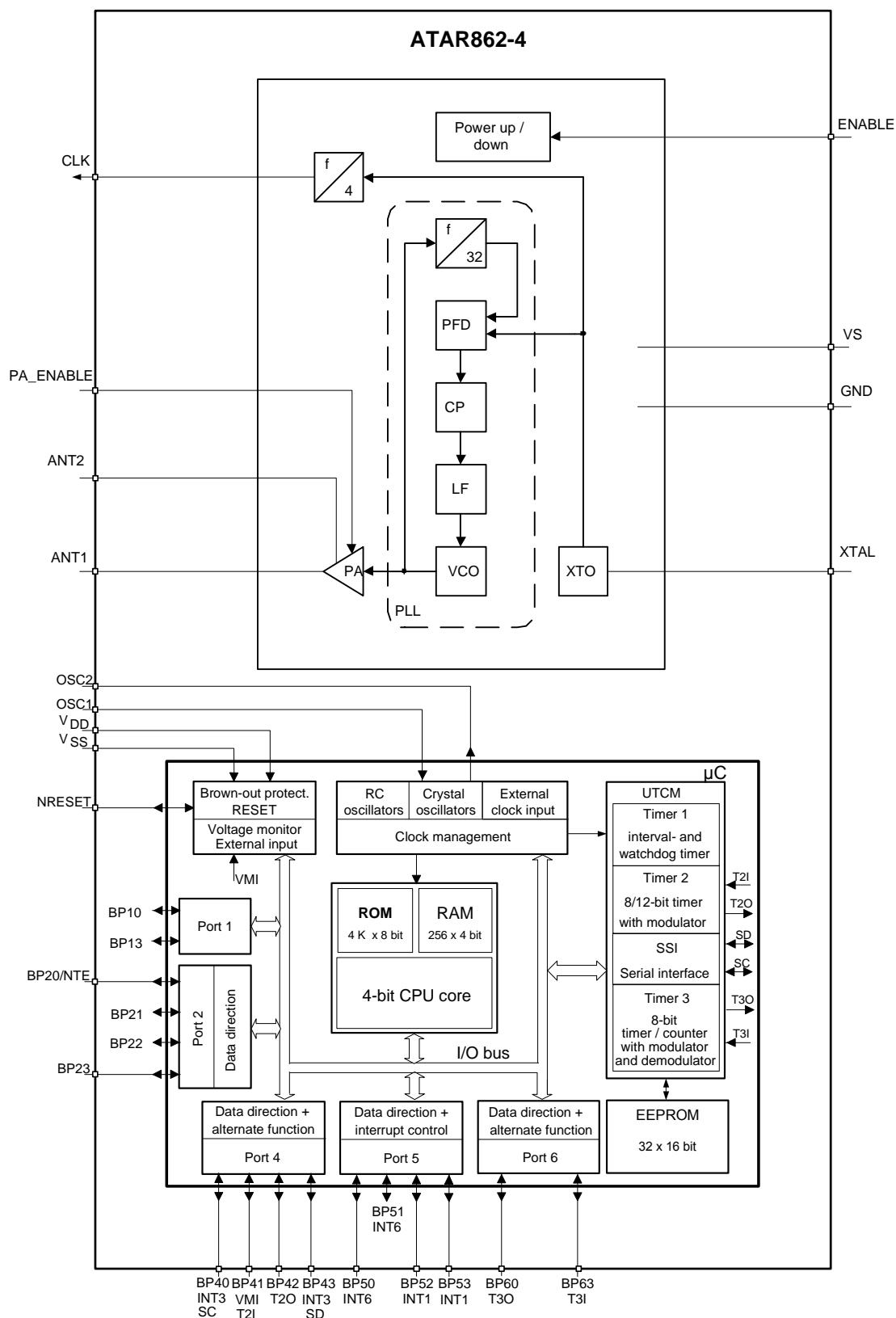
Figure 3. Block Diagram
