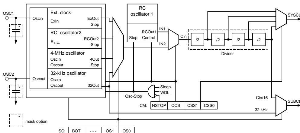
Figure 21. Clock Module
