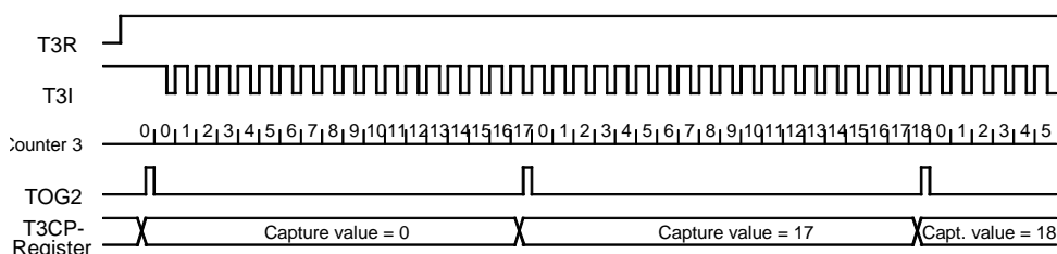
Figure 86. Frequency Measurement
