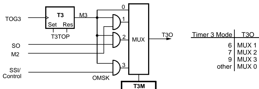
Figure 62. Modulator 3
