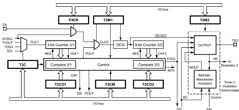
Figure 36. Timer 2
