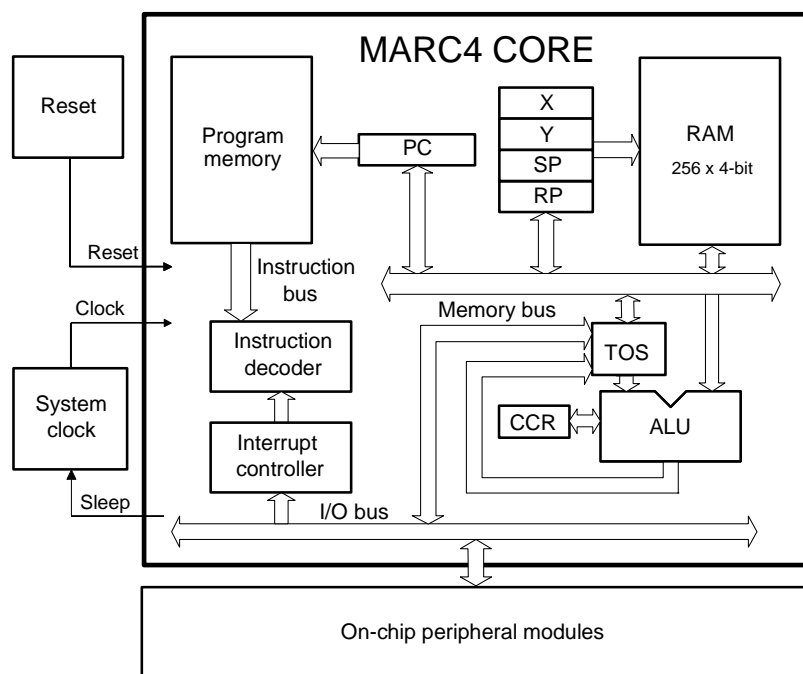
Figure 10. MARC4 Core
