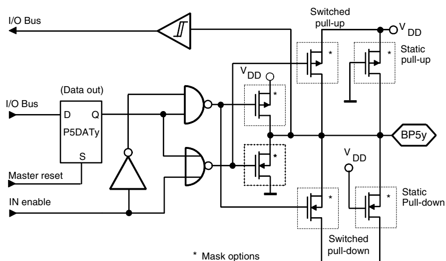
Figure 23. Bi-directional Port 5
