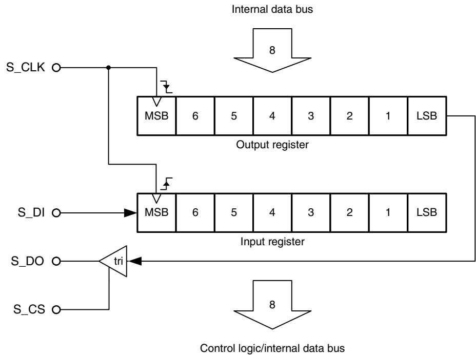
Figure 8. SPI Structure
