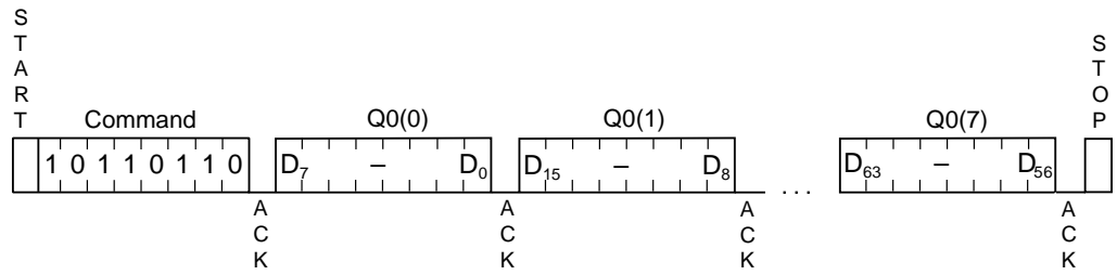
Figure 11. Initialize Authentication
