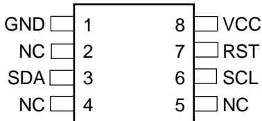
8-pin SOIC, PDIP, or LAP
