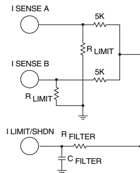
FIGURE B. CURRENT LIMIT WITH SHUTDOWN CURRENT MODE.
