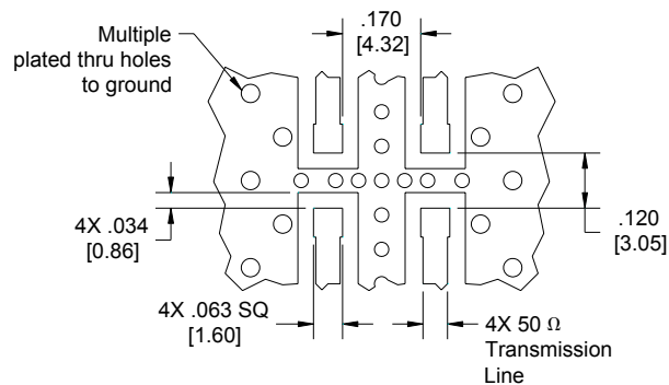
Dimensions are in Inches [Millimeters] 1P510 Rev A Mounting Footprint
