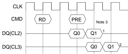
1) Read Interrupted by Precharge (BL=4)
