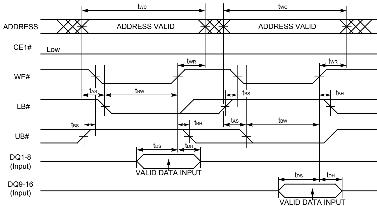
Figure II.29. Asynchronous Write Timing #3-2 (WE# / LB# / UB# Byte Write Control)
