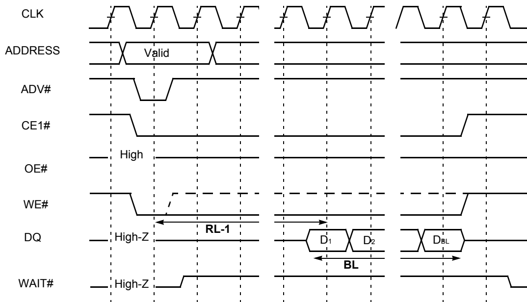
Figure II.II. Burst Write Operation
