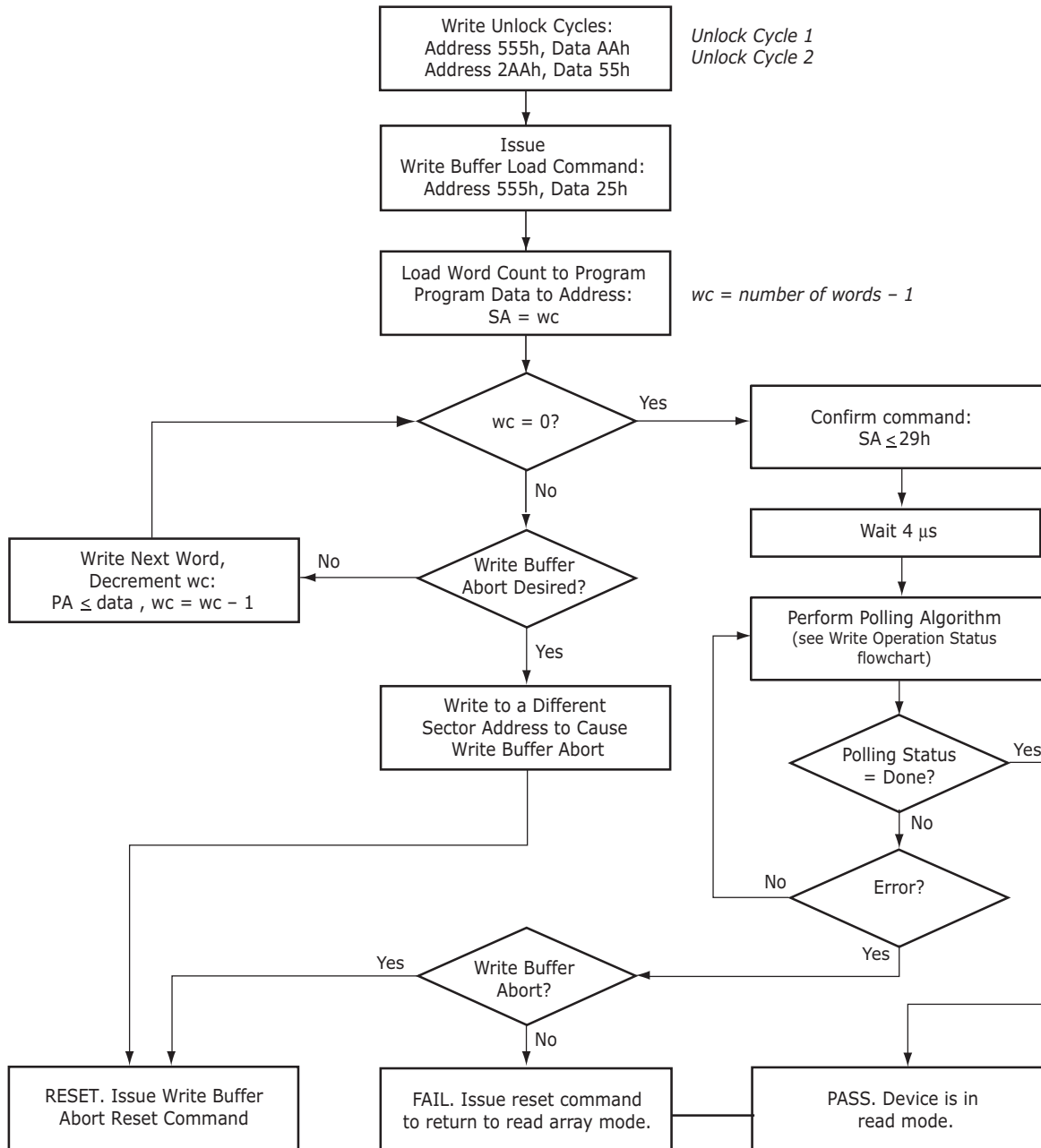
Figure 5.22. Write Buffer Programming Operation
