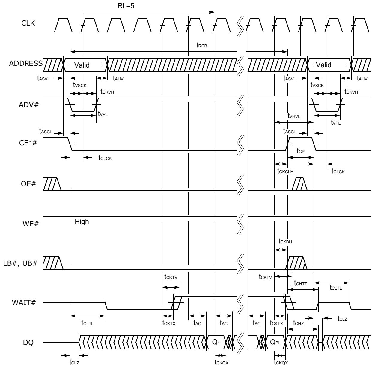
Figure II.39. 32M Synchronous Read Timing #2 (CE1# Control)
