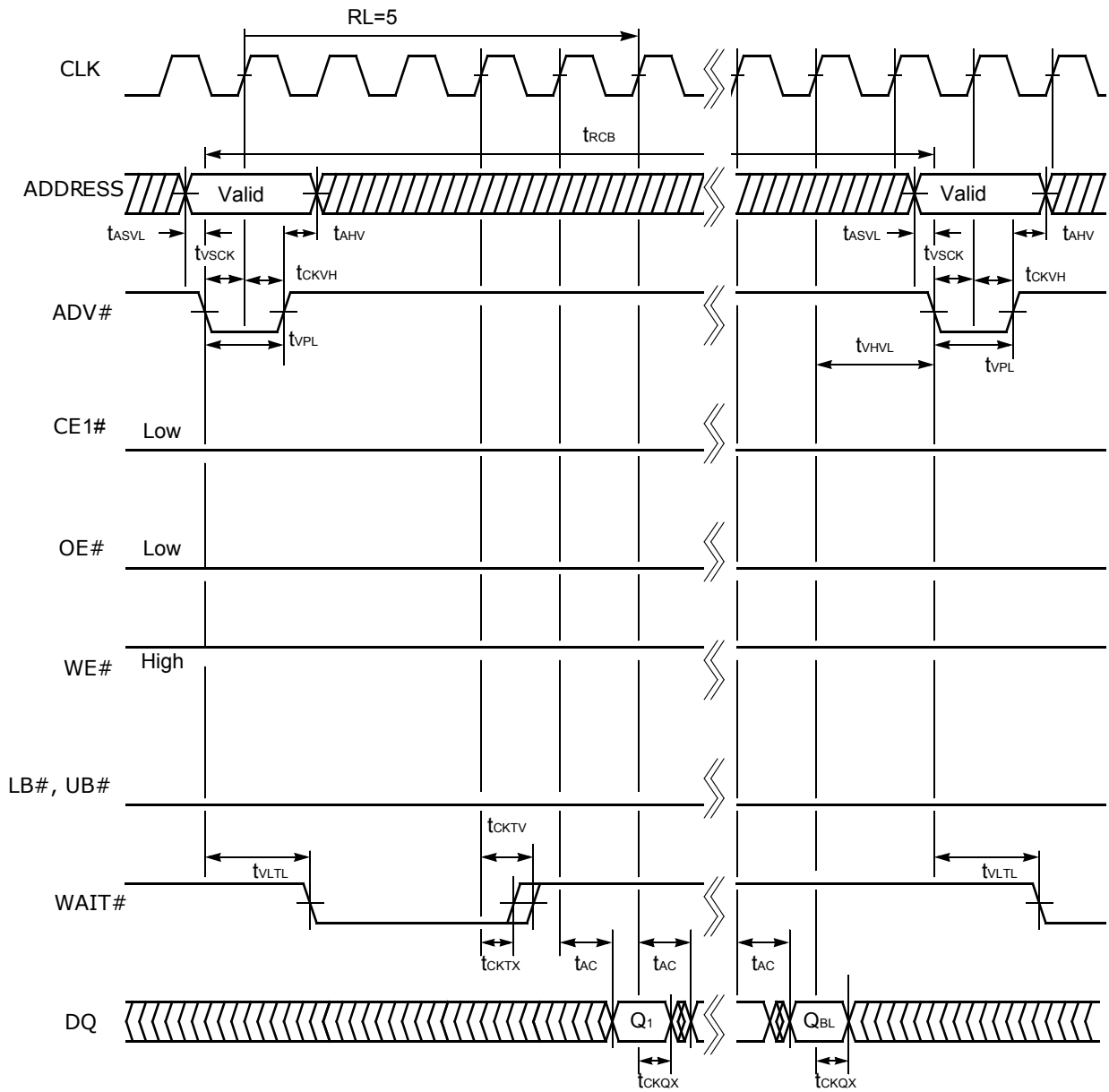
Figure II.44. 64M Synchronous Read Timing #3 (ADV# Control)
