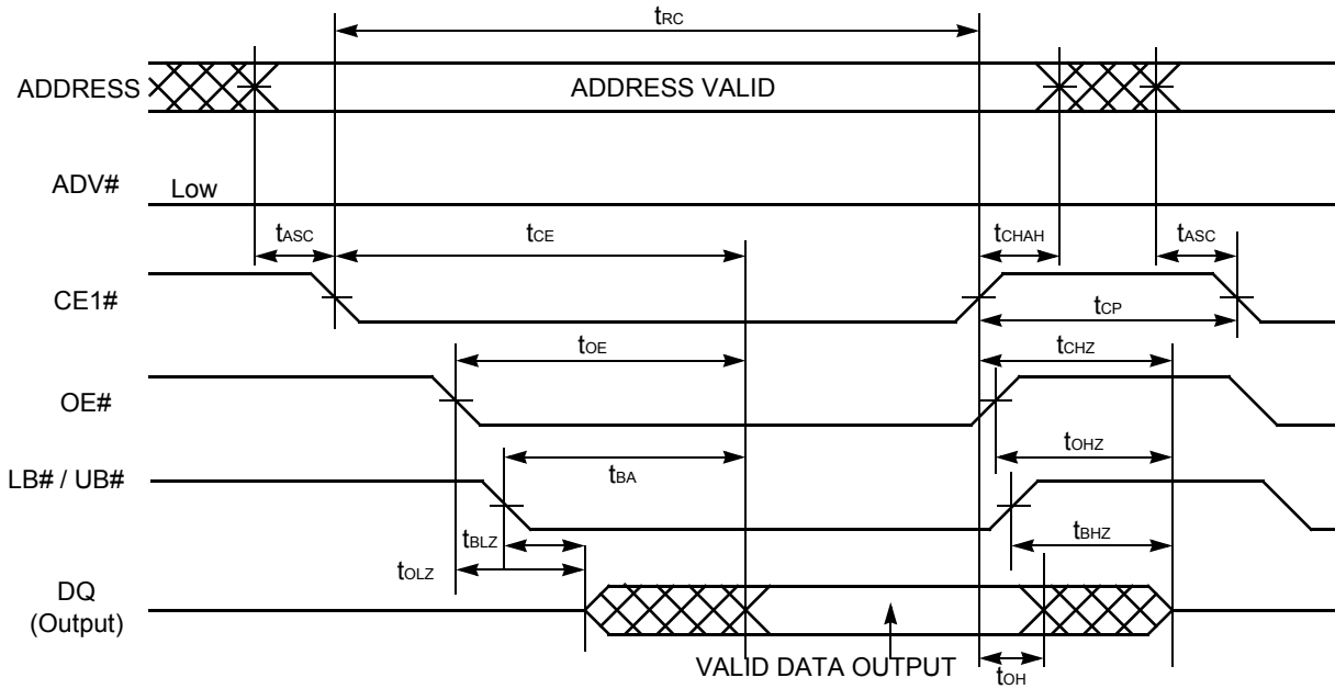
Figure II.19. Asynchronous Read Timing #1-1 (Basic Timing)
