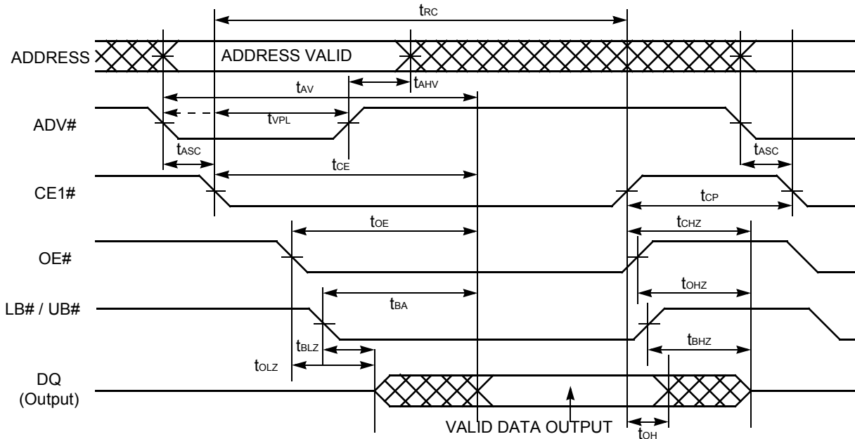
Figure II.20. Asynchronous Read Timing #1-2 (Basic Timing)
