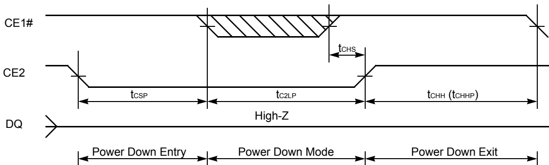
Figure II.57. Power Down Entry and Exit Timing
