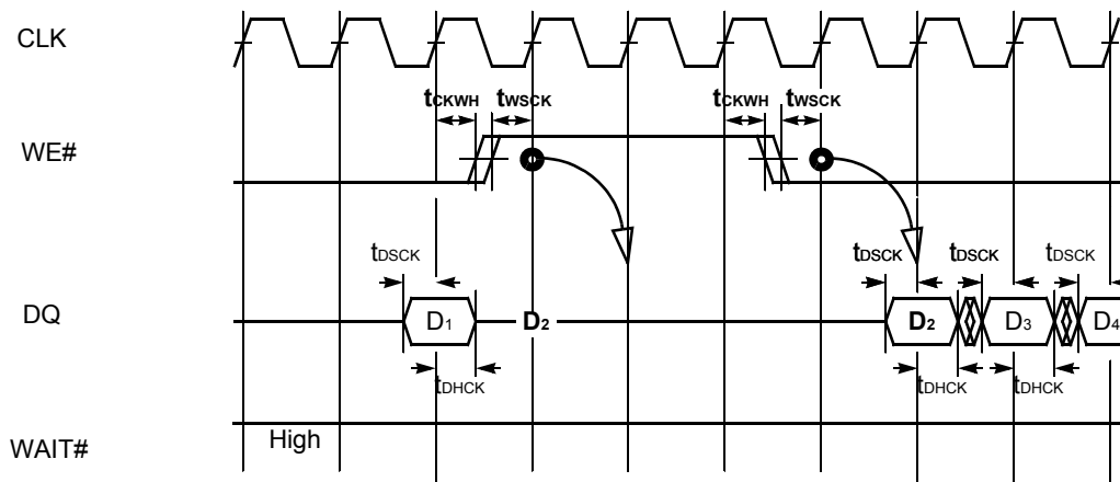
Figure II.15. Burst Write Suspend Diagram
