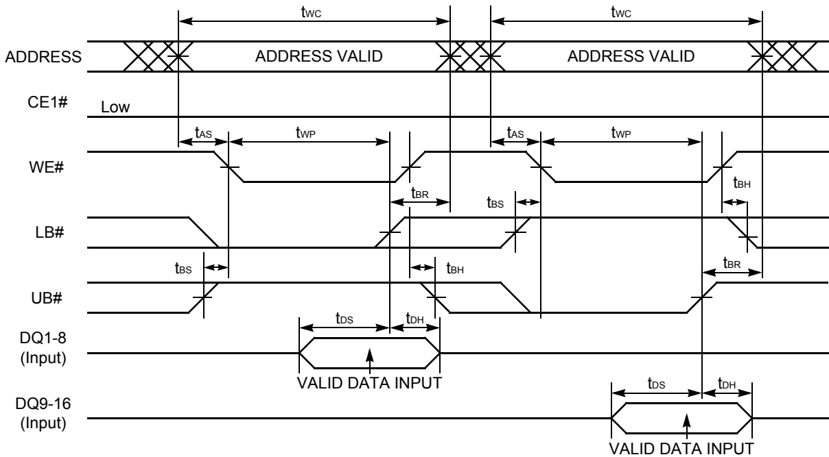
Figure II.28. Asynchronous Write Timing #3-I (WE# / LB# / UB# Byte Write Control)
