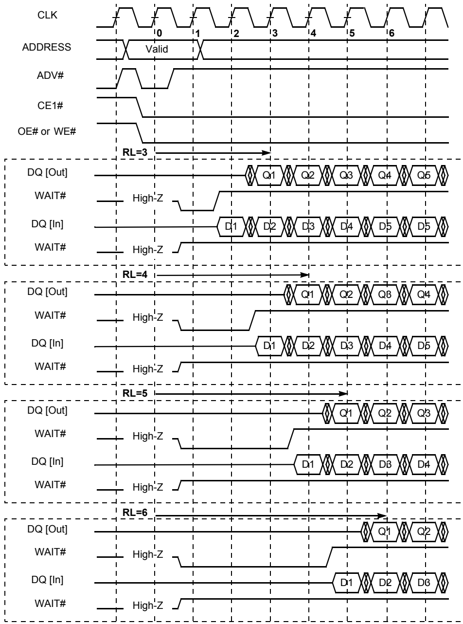
Figure II.I2. Read Latency Diagram
