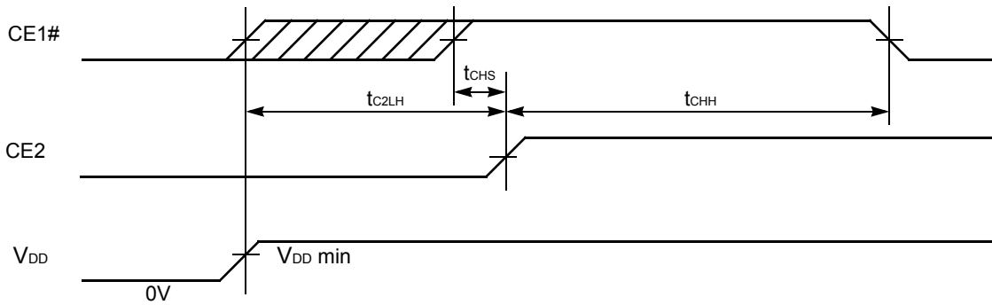
Figure II.55. Power-up Timing #1
