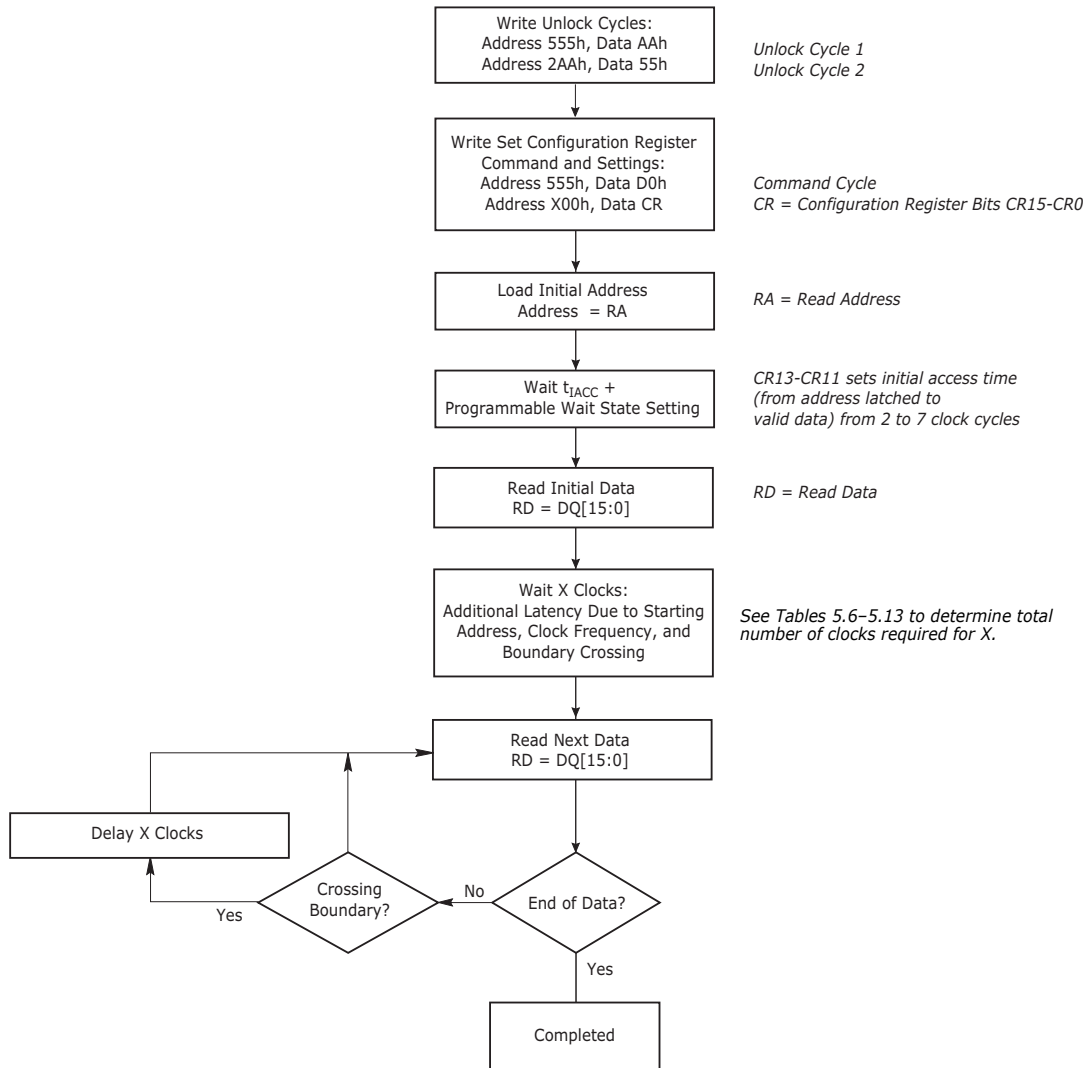
Figure 5.2. Synchronous Read
