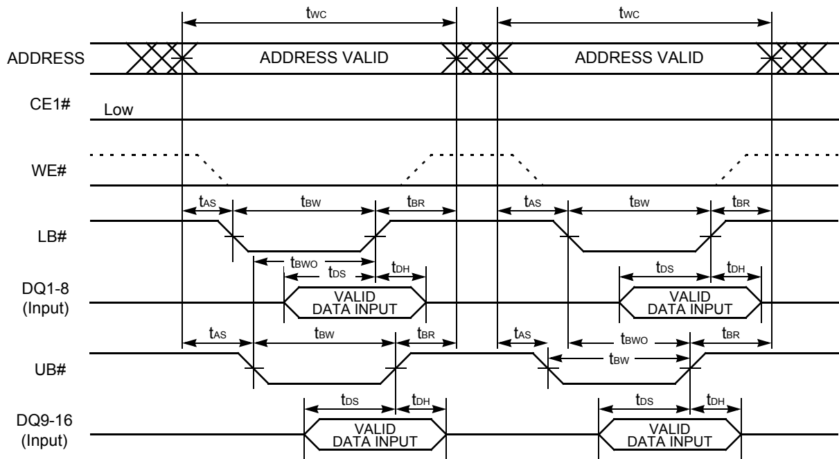
Figure II.31. Asynchronous Write Timing #3-4 (WE# / LB# / UB# Byte Write Control)
