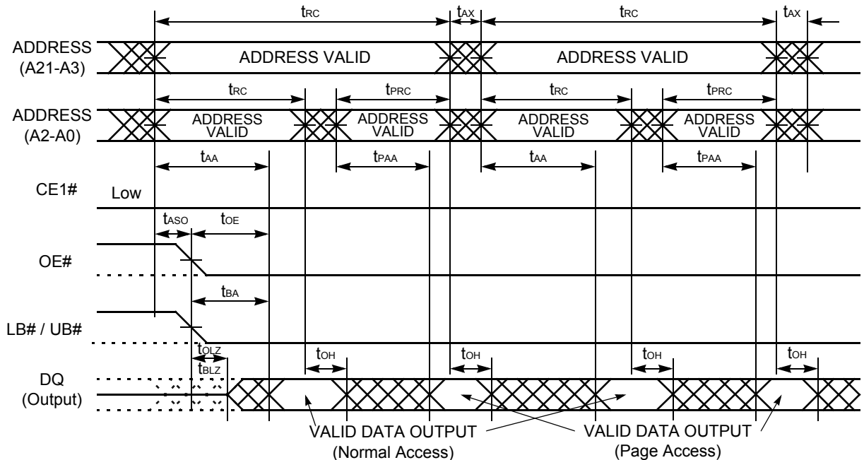
Figure II.24. Asynchronous Read Timing #5 (Random and Page Address Access)
