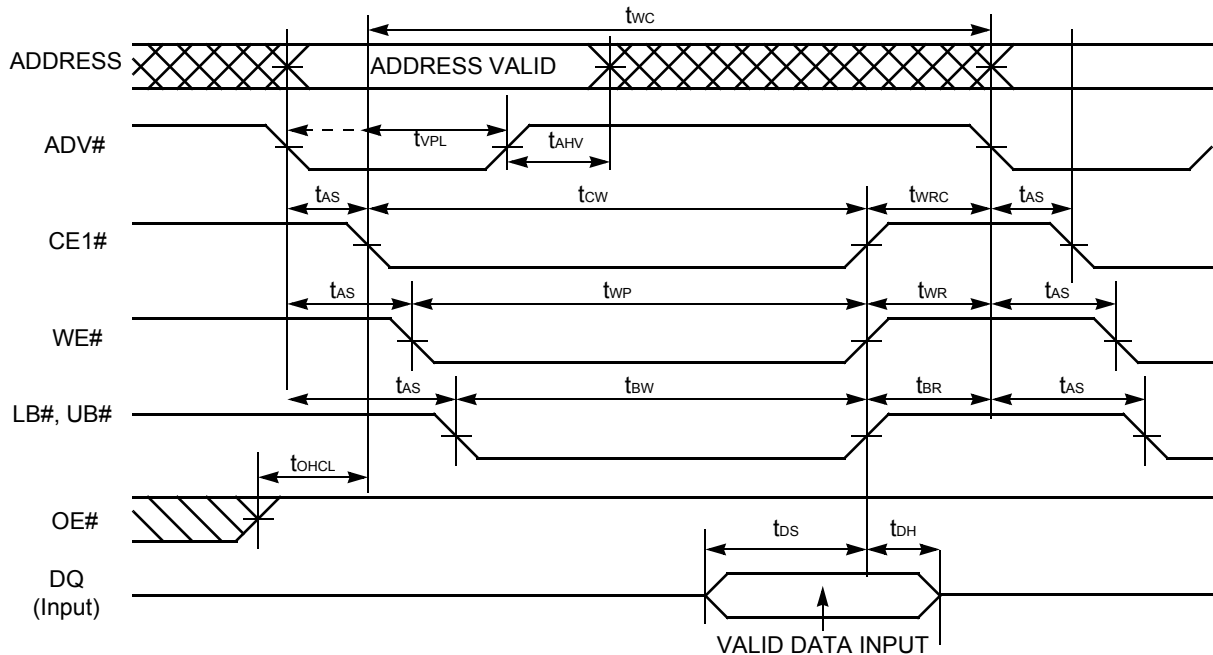
Figure II.26. Asynchronous Write Timing #1-2 (Basic Timing)
