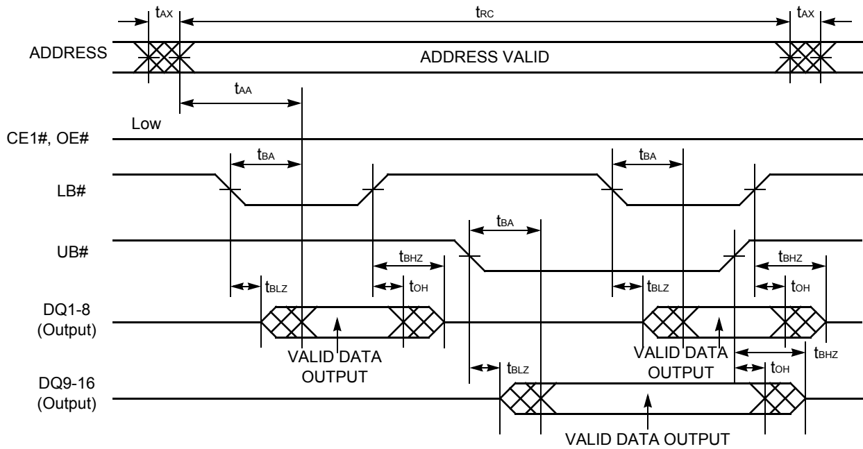
Figure II.22. Asynchronous Read Timing #3 (LB# / UB# Byte Access)
