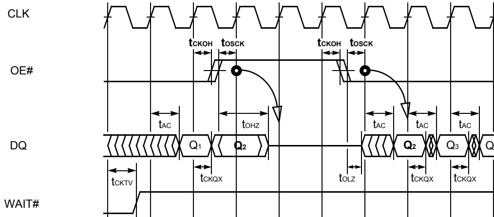
Figure II.14. Burst Read Suspend Diagram
