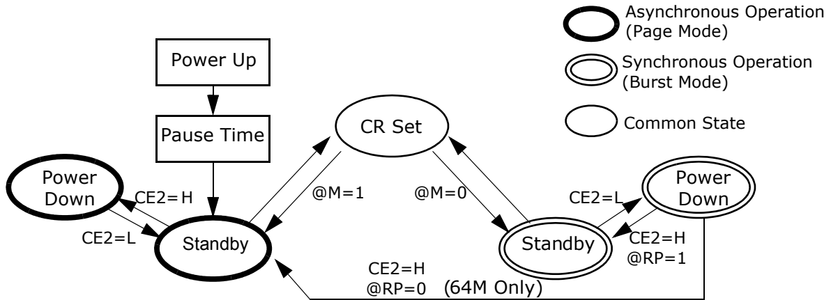
Figure II.7. Initial Standby State Diagram
