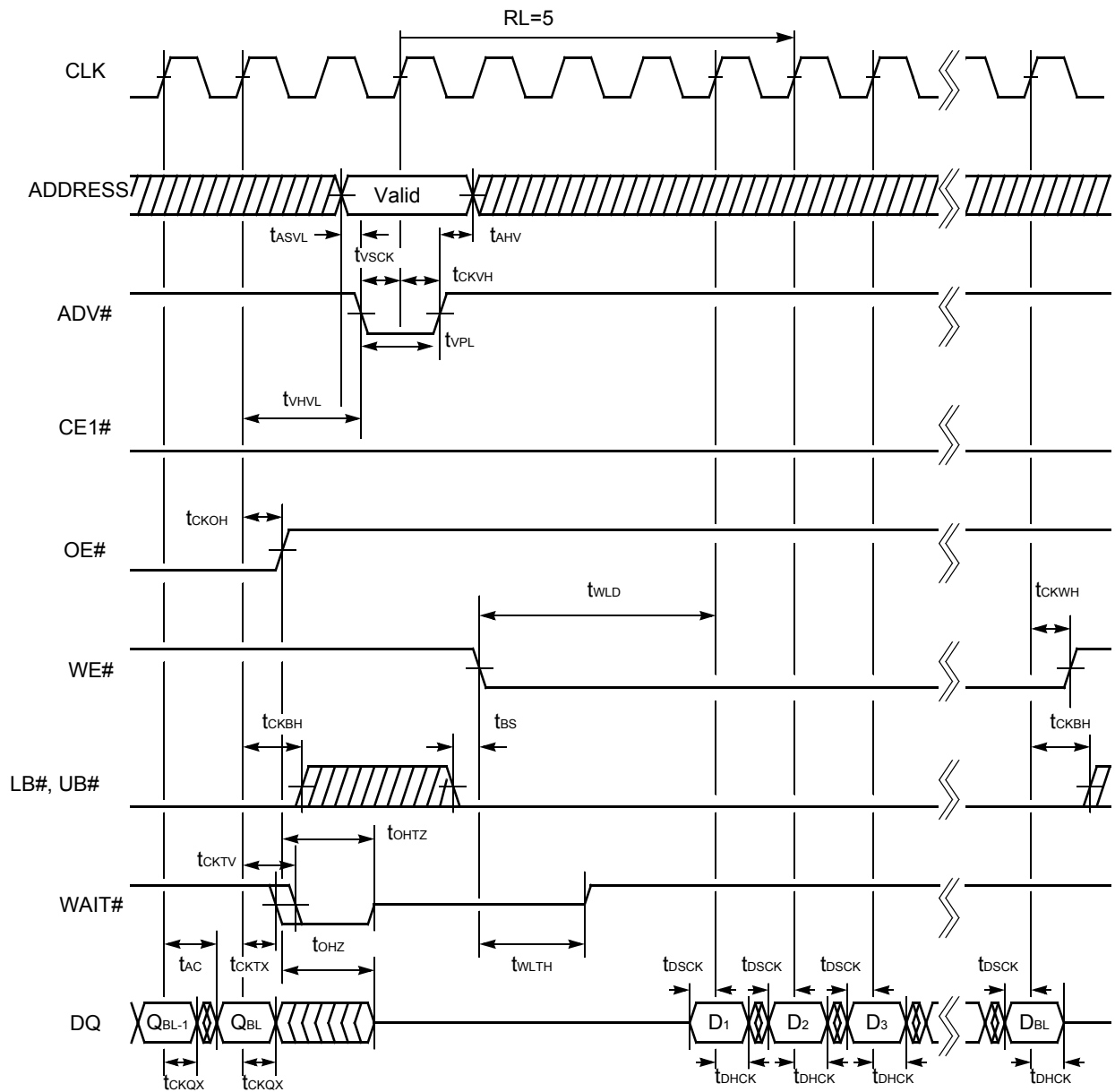
Figure II.50. 32M Synchronous Read to Write Timing #2(ADV# Control)
