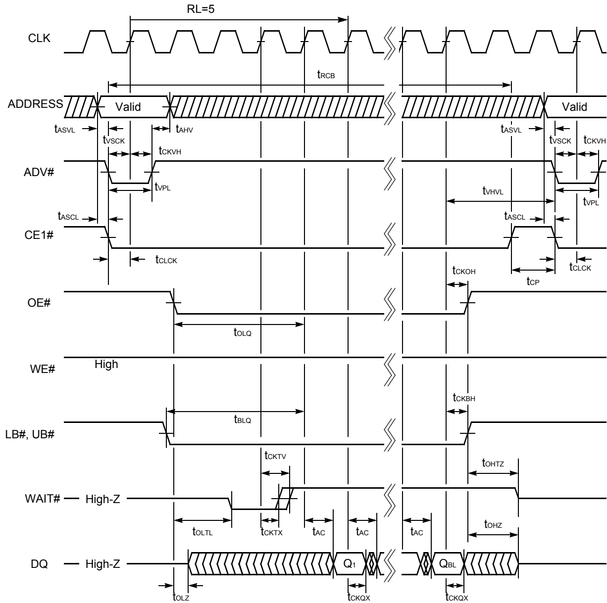
Figure II.42. 64M Synchronous Read Timing #1 (OE# Control)
