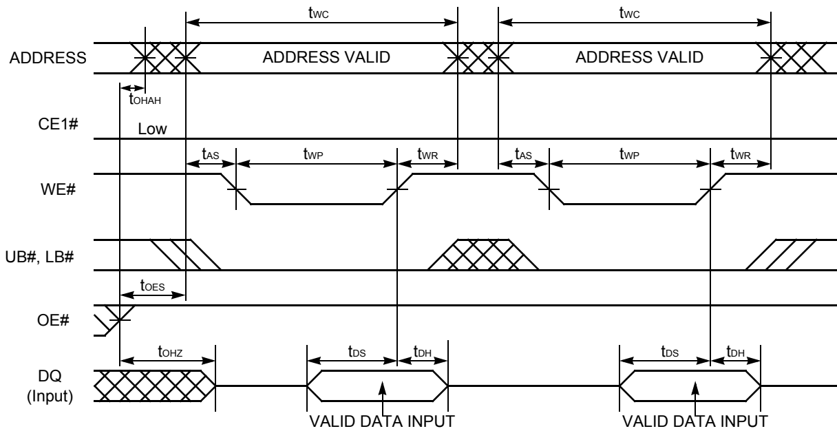
Figure II.27. Asynchronous Write Timing #2 (WE# Control)
