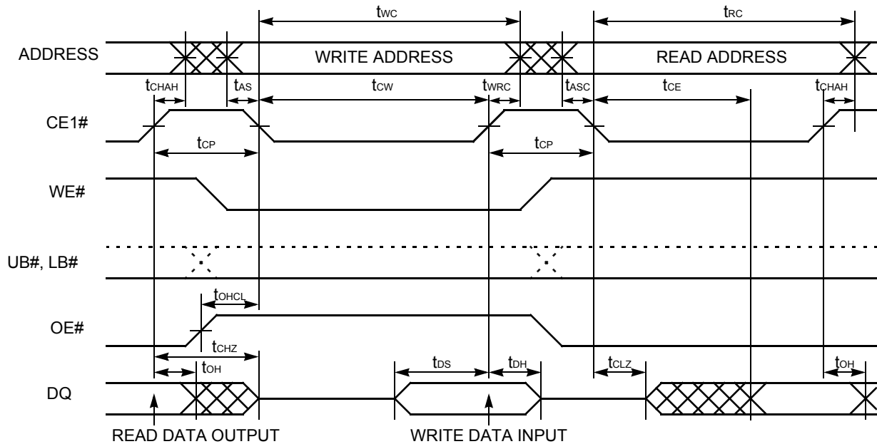
Figure II.32. Asynchronous Read / Write Timing #1-1 (CE1# Control)
