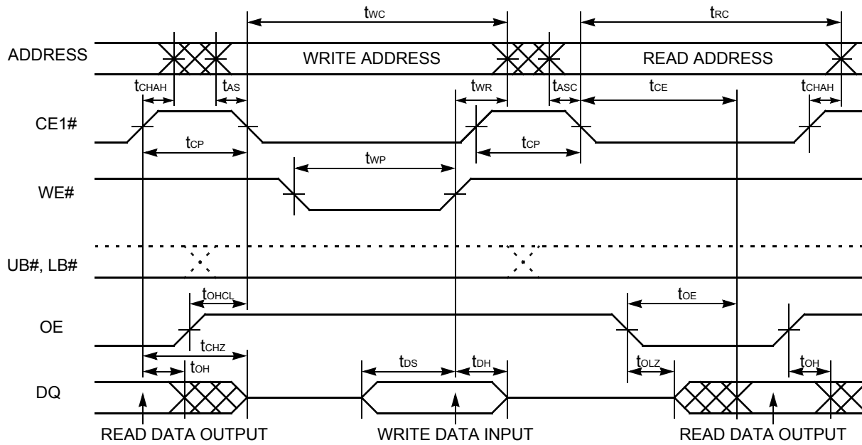
Figure II.33. Asynchronous Read / Write Timing #1-2 (CE1# / WE# / OE# Control)
