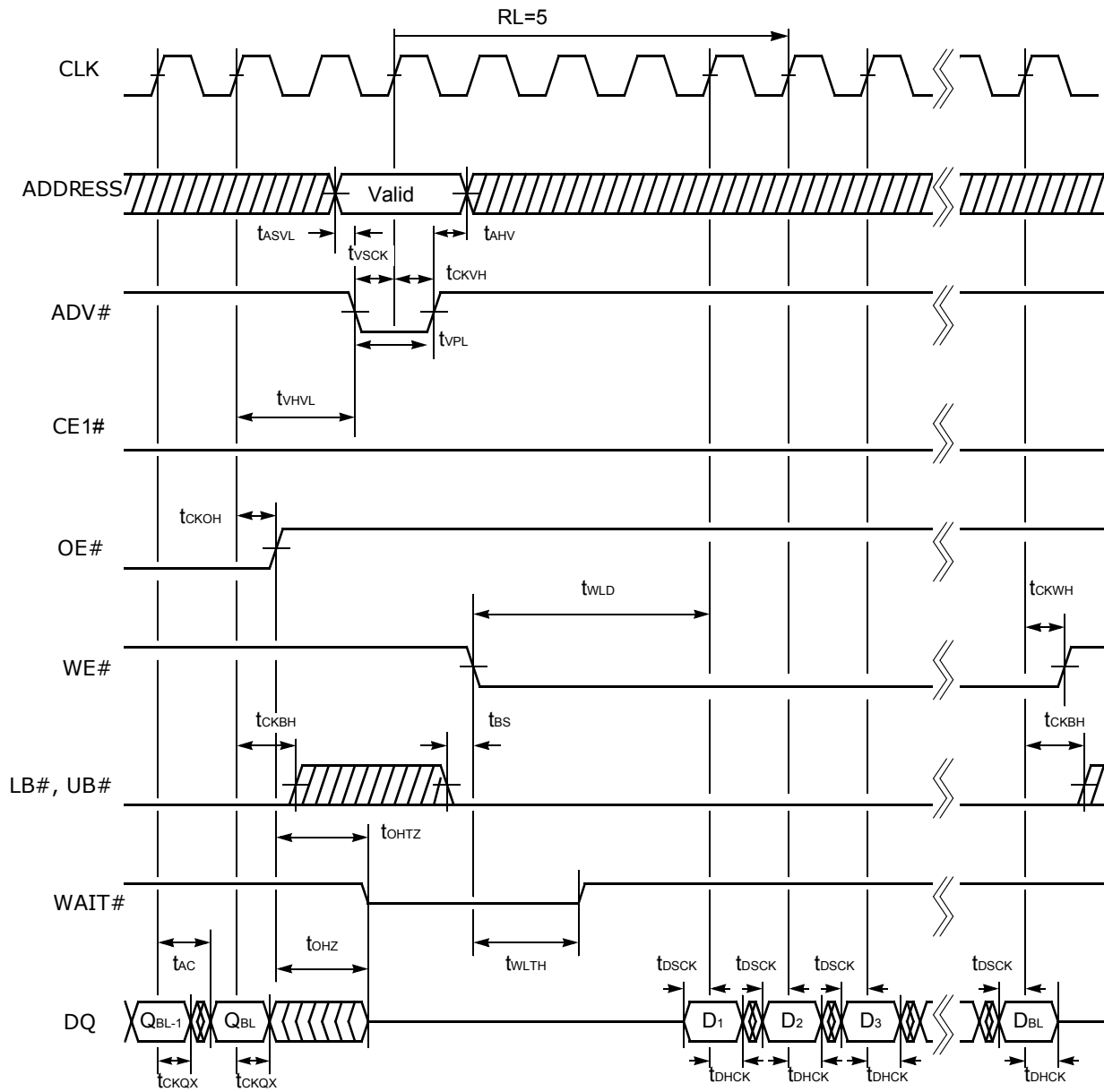
Figure II.52. 64M Synchronous Read to Write Timing #2(ADV# Control)
