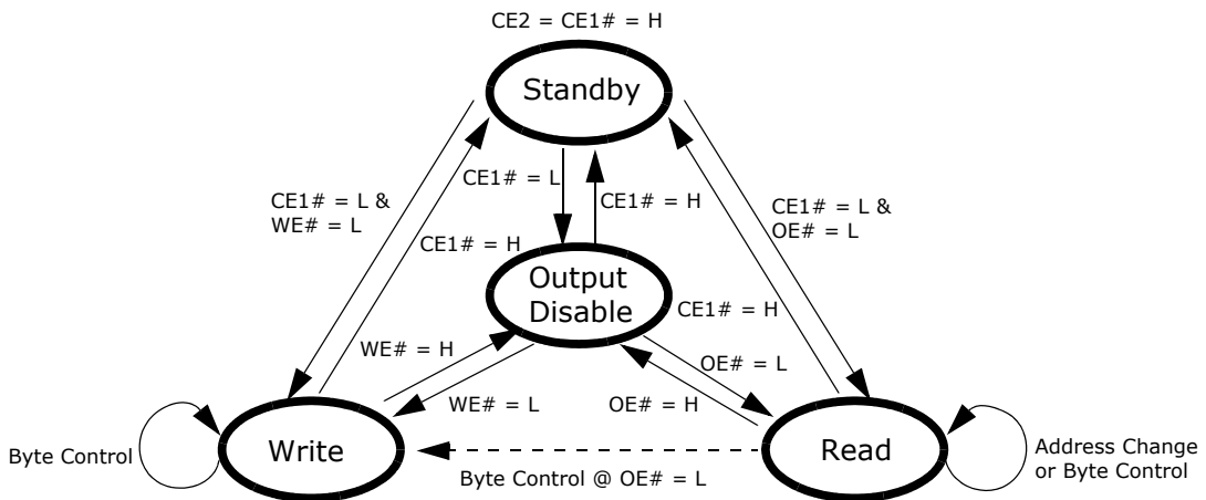
Figure II.8. Asynchronous Operation State Diagram
