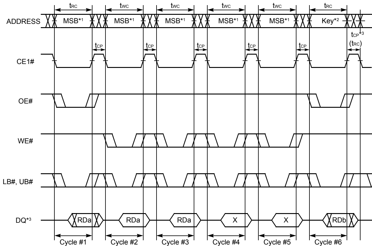
Figure II.59. Configuration Register Set Timing #1 (Asynchronous Operation)
