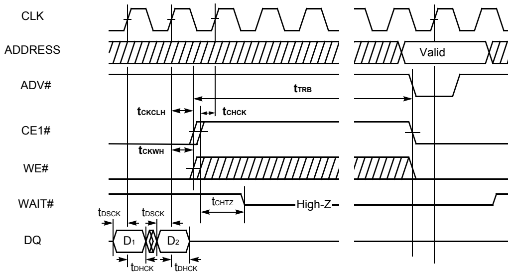
Figure II.17. Burst Write Termination Diagram
