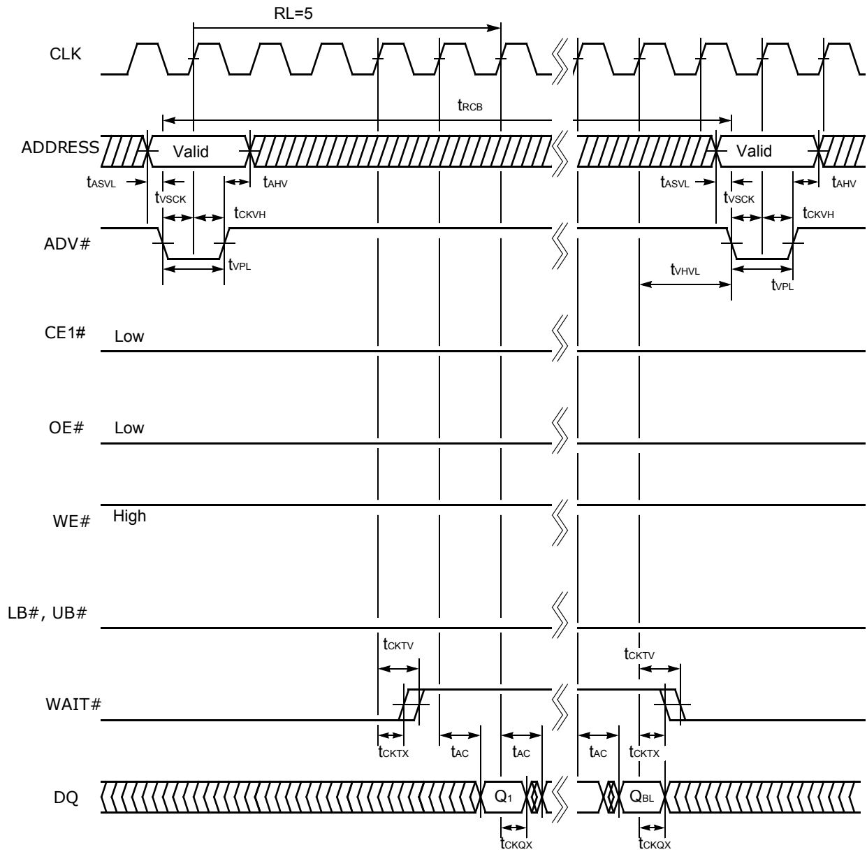
Figure II.40. 32M Synchronous Read Timing #3 (ADV# Control)
