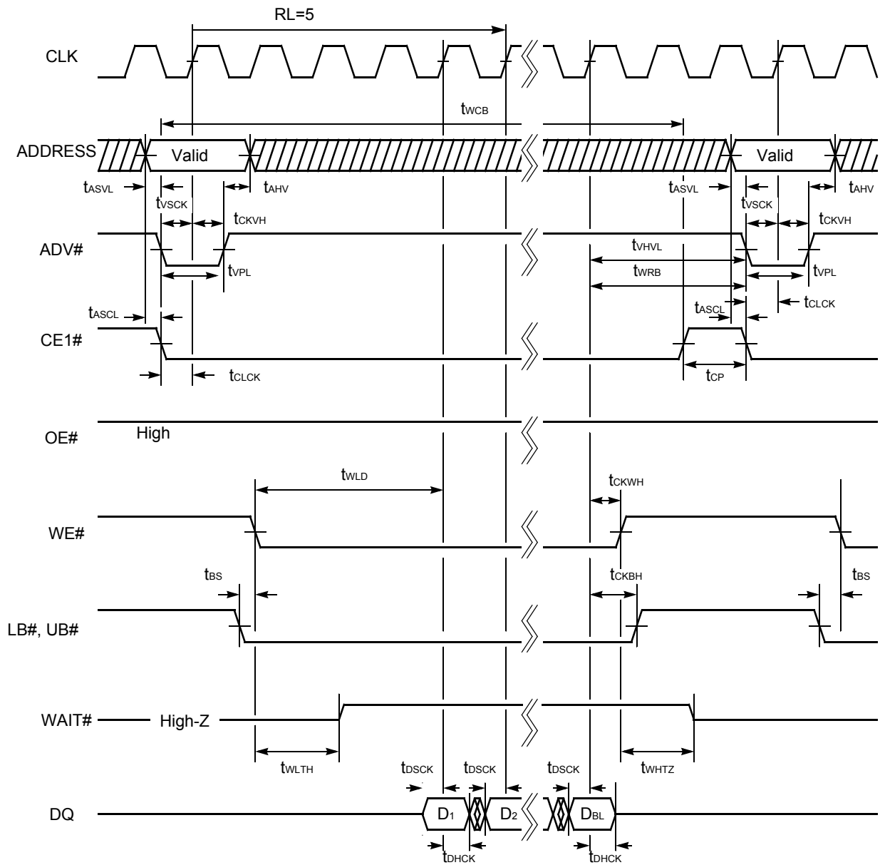
Figure II.45. Synchronous Write Timing #1 (WE# Level Control)
