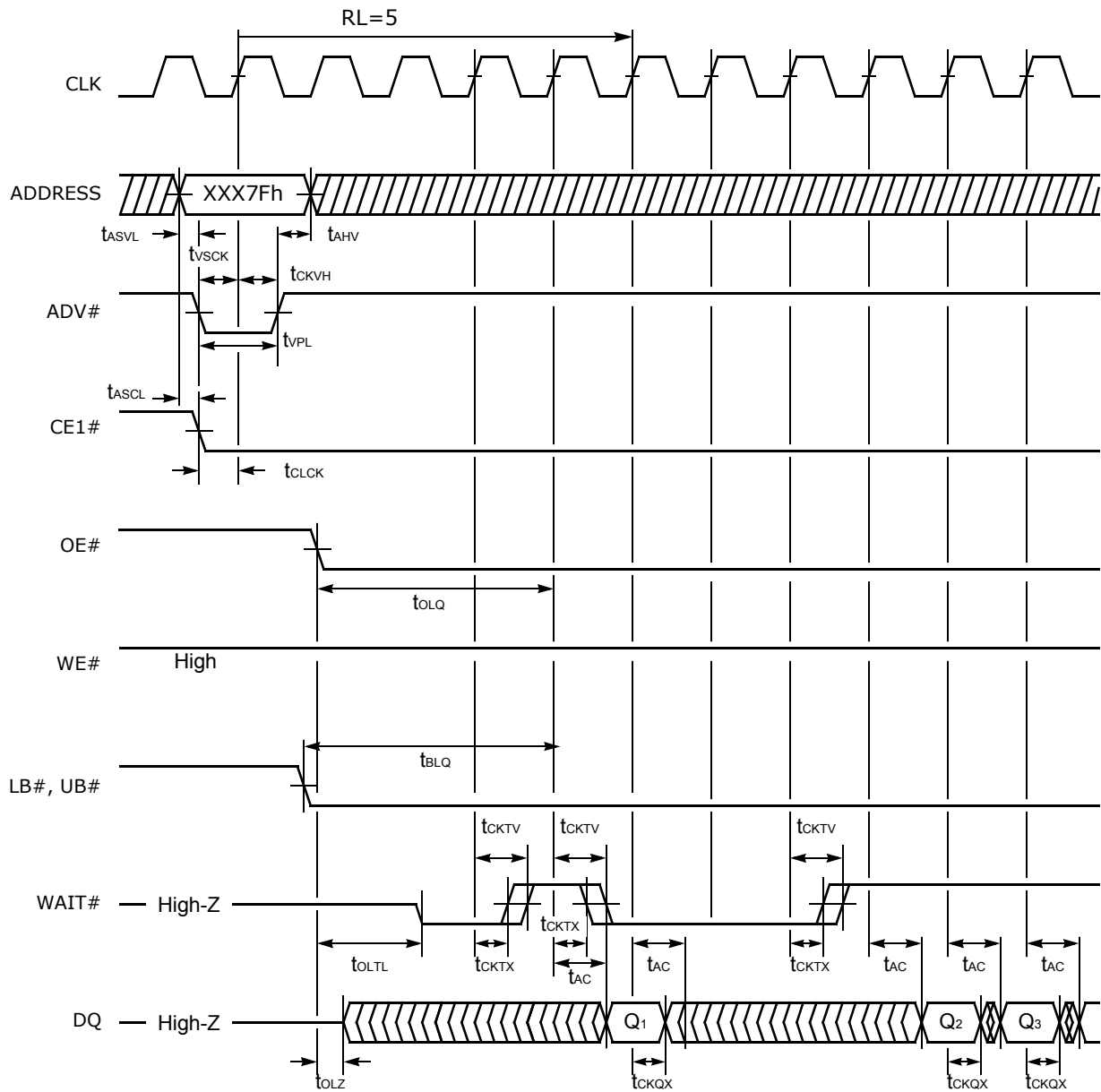
Figure II.4I. Synchronous Read - WAIT# Output Timing (Continuous Read)
