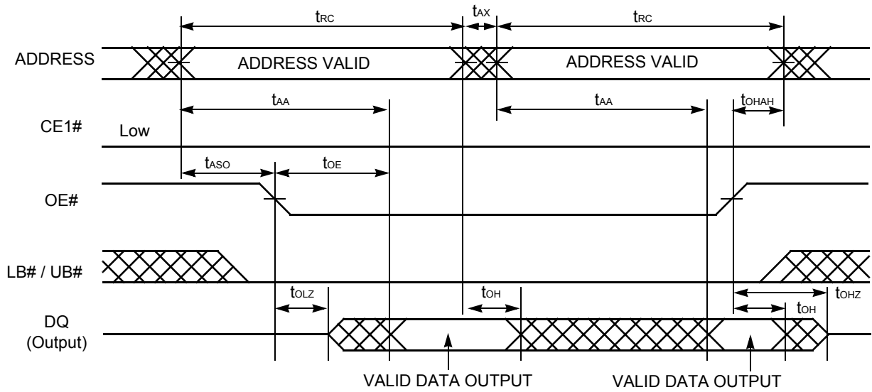
Figure II.21. Asynchronous Read Timing #2 (OE# & Address Access)
