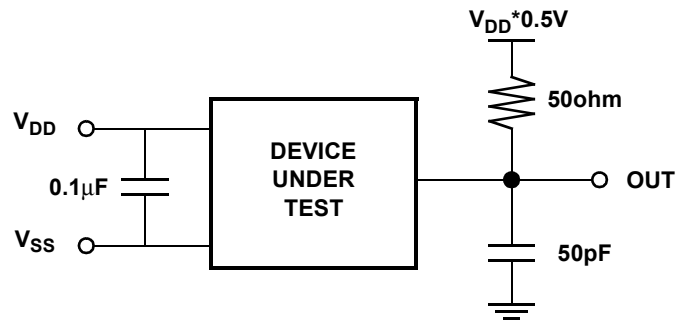
Figure 11.18. Output Load Circuit
