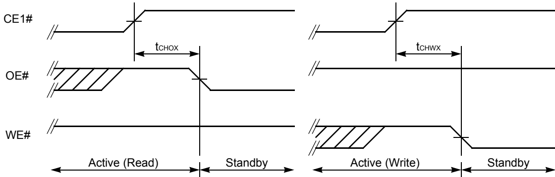
Figure II.58. Standby Entry Timing after Read or Write
