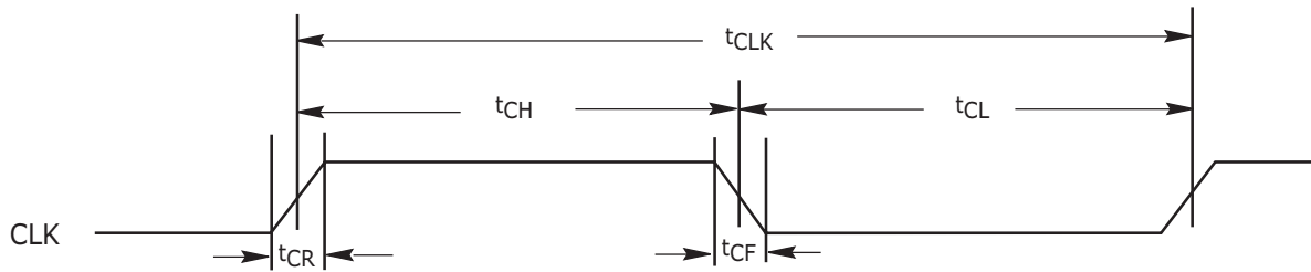
Figure 9.6. CLK Characterization
