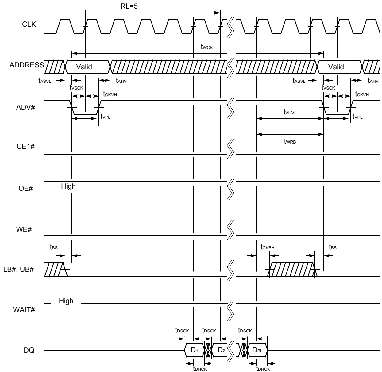
Figure II.47. Synchronous Write Timing #3 (ADV# Control)
