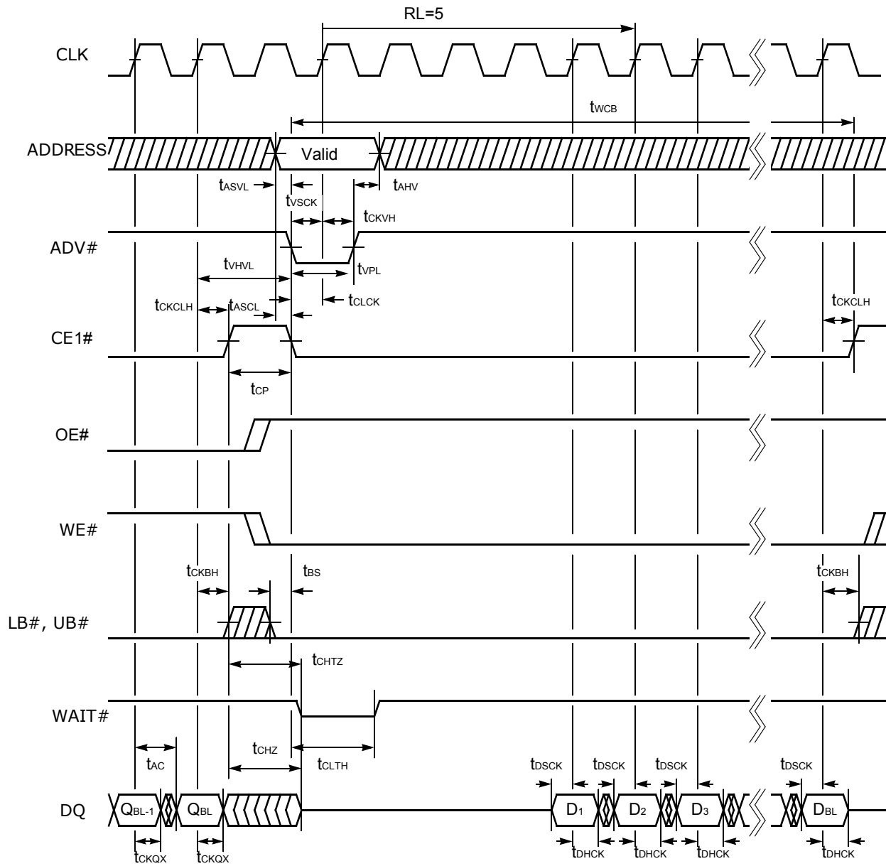
Figure II.51. 64M Synchronous Read to Write Timing #I(CE1# Control)
