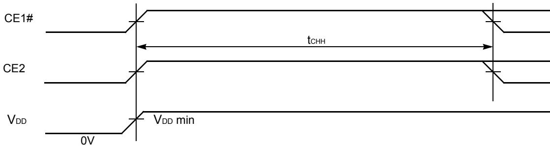
Figure II.56. Power-up Timing #2
