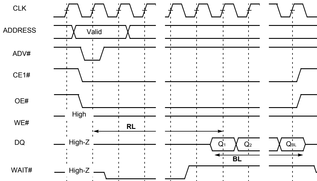
Figure II.I0. Burst Read Operation
