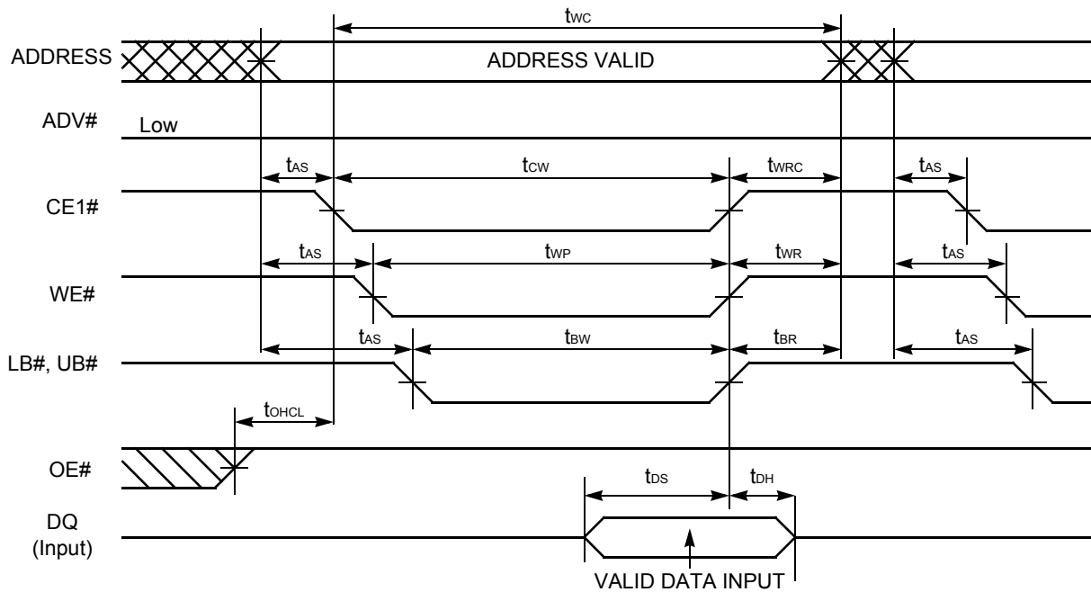
Figure II.25. Asynchronous Write Timing #1-1 (Basic Timing)
