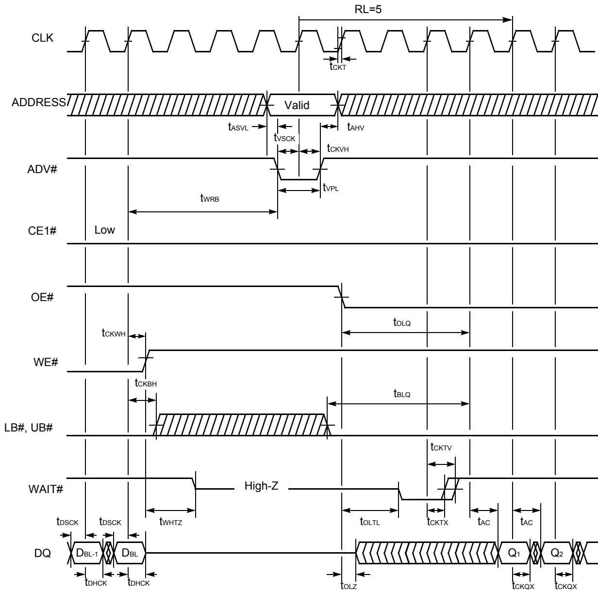
Figure II.54. Synchronous Write to Read Timing #2 (ADV# Control)
