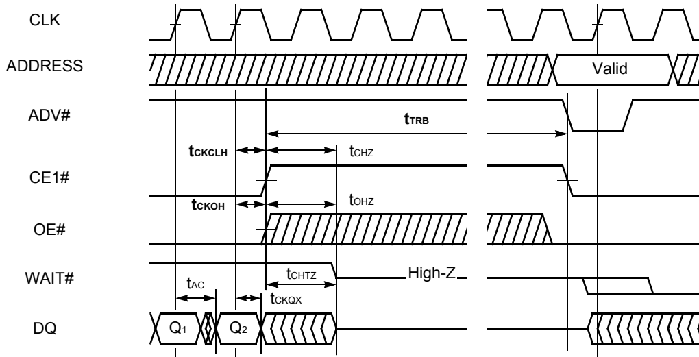
Figure II.16. Burst Read Termination Diagram
