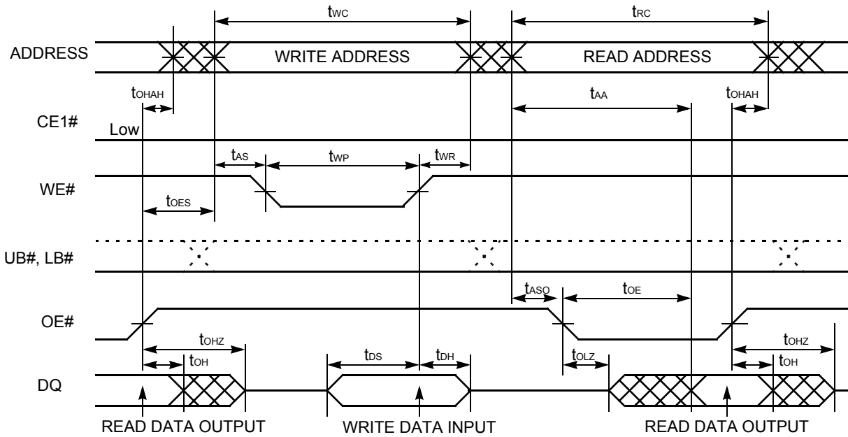
Figure II.34. Asynchronous Read / Write Timing #2 (OE#, WE# Control)
