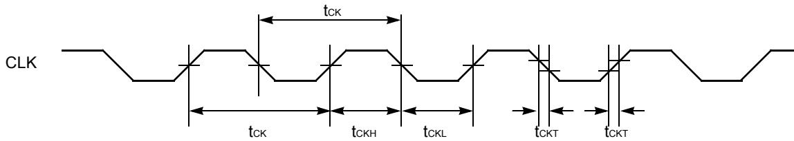
Figure II.36. Clock Input Timing
