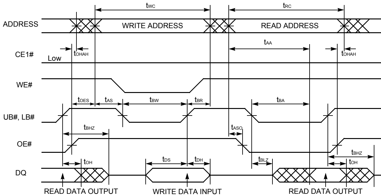
Figure II.35. Asynchronous Read / Write Timing #3 (OE,# WE#, LB#, UB# Control)
