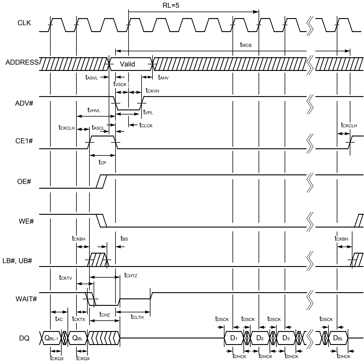
Figure II.49. 32M Synchronous Read to Write Timing #1(CE1# Control)
