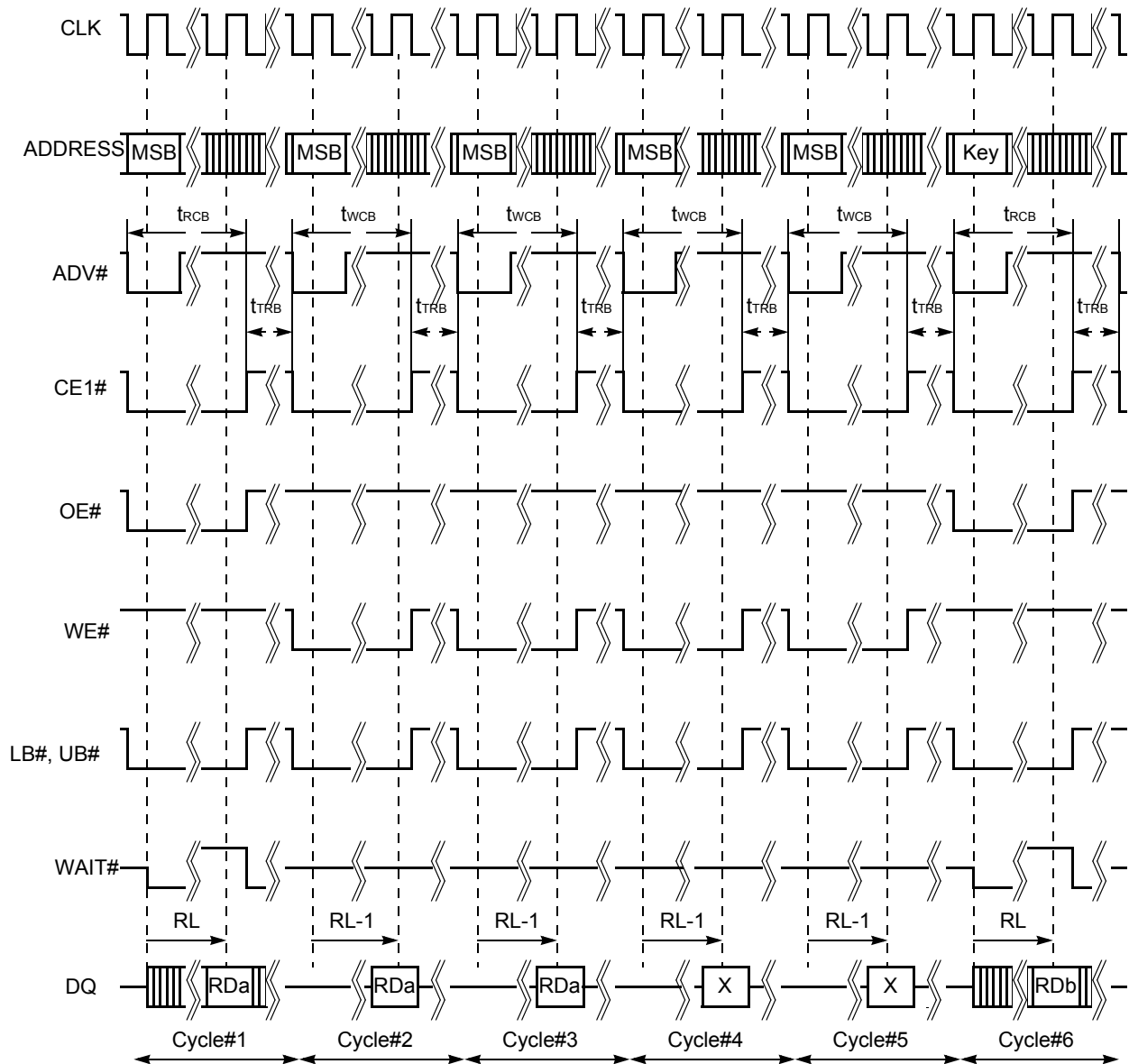
Figure II.60. Configuration Register Set Timing #2 (Synchronous Operation)
