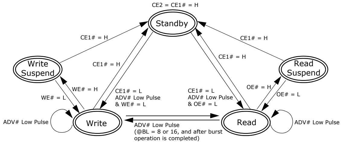
Figure II.9. Synchronous Operation Diagram
