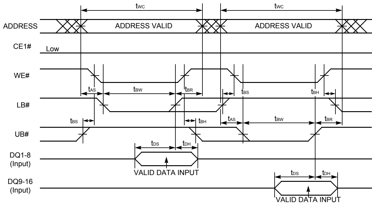
Figure II.30. Asynchronous Write Timing #3-3 (WE# / LB# / UB# Byte Write Control)
