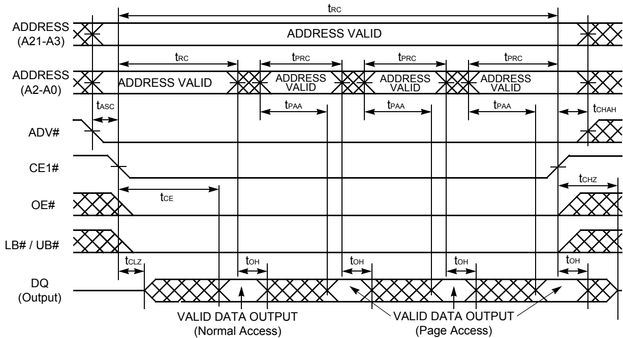
Figure II.23. Asynchronous Read Timing #4 (Page Address Access after CE1# Control Access)
