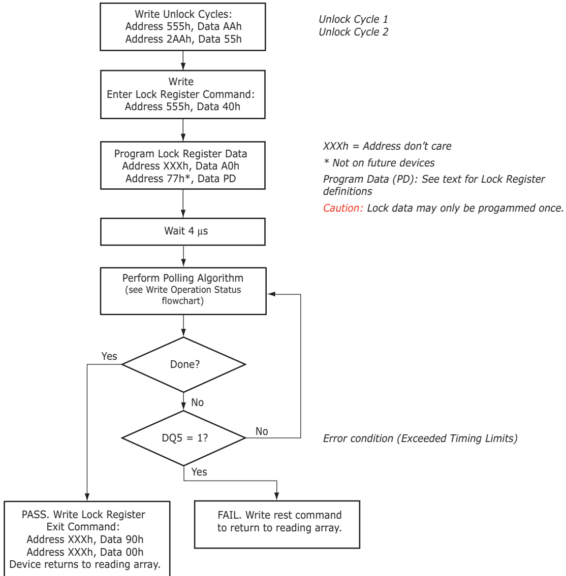
Figure 6.2. Lock Register Program Algorithm
