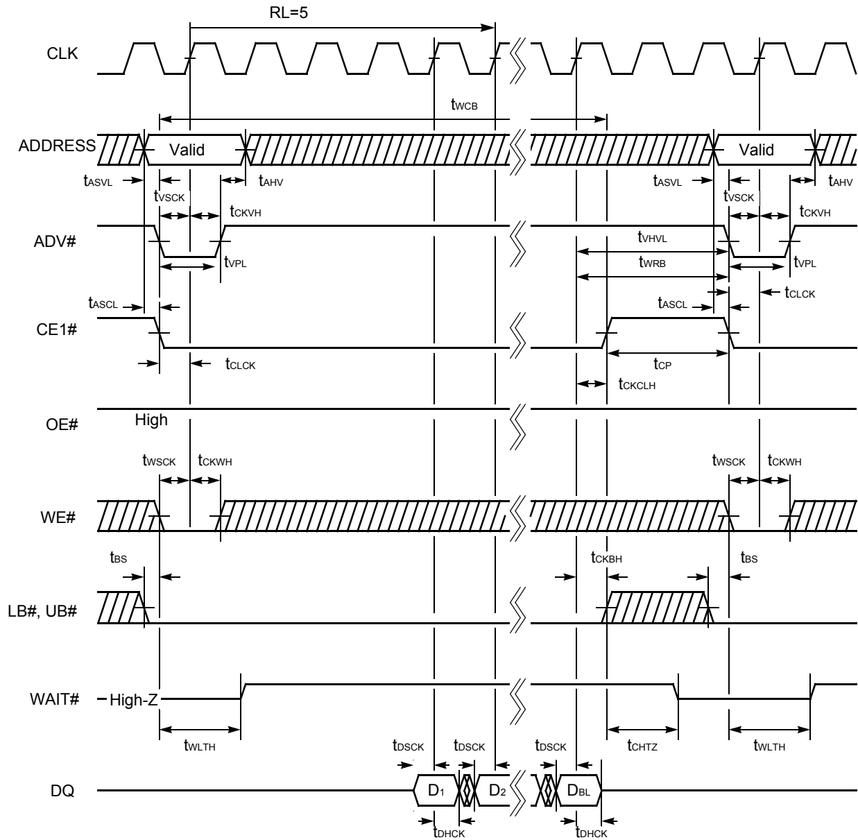
Figure II.46. Synchronous Write Timing #2 (WE# Single Clock Pulse Control)
