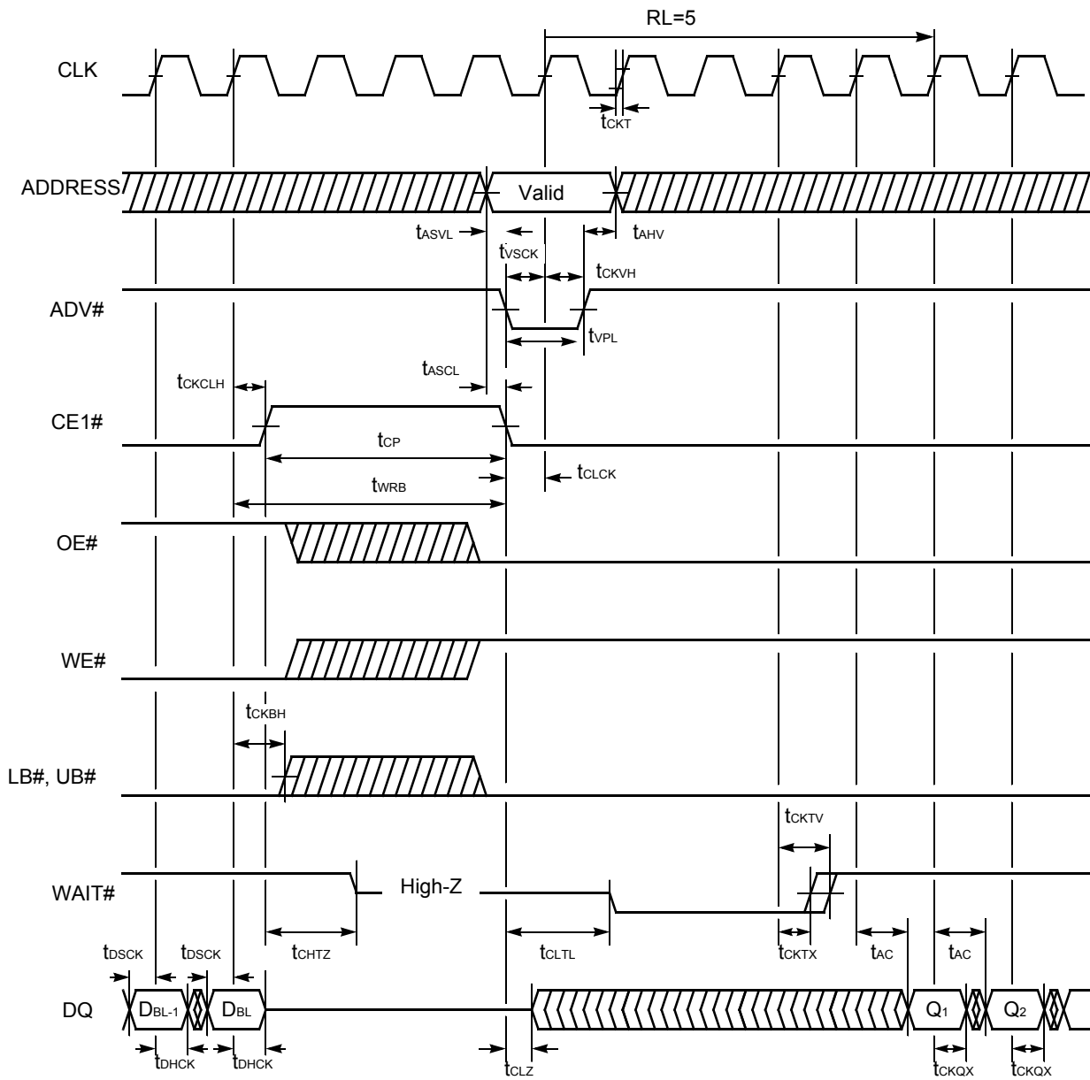
Figure II.53. Synchronous Write to Read Timing #1 (CE1# Control)
