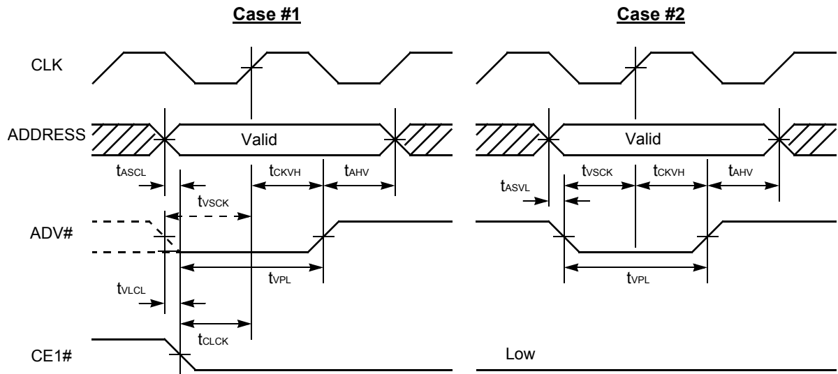
Figure II.37. Address Latch Timing (Synchronous Mode)
