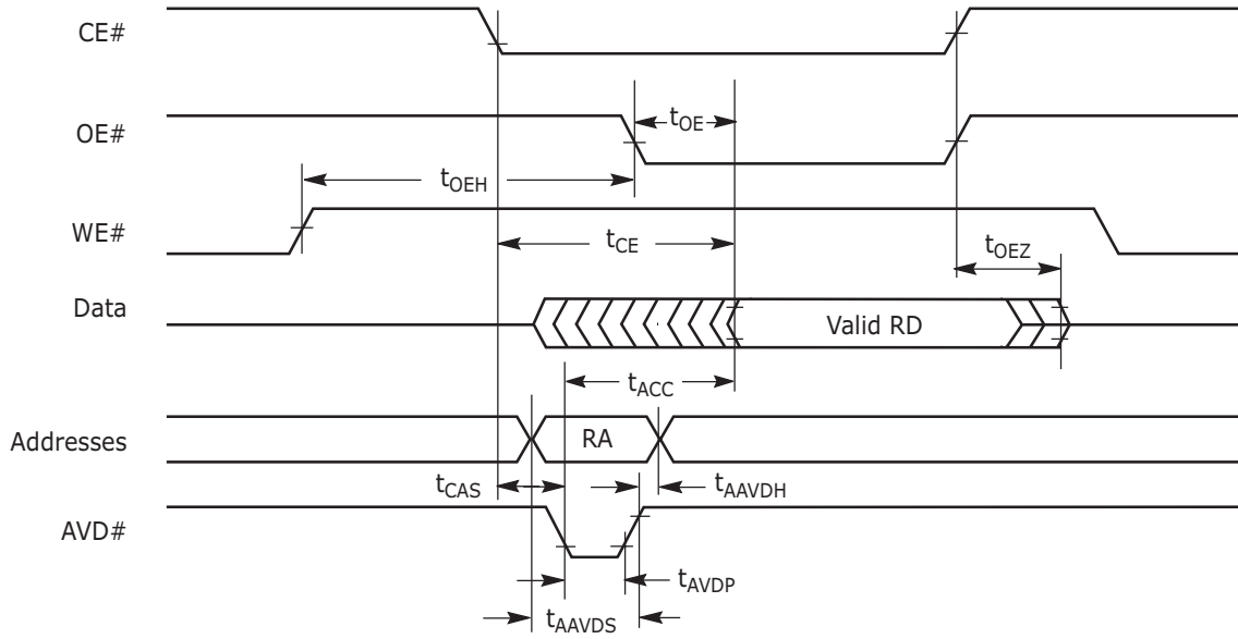
Figure 9.II. Asynchronous Mode Read
