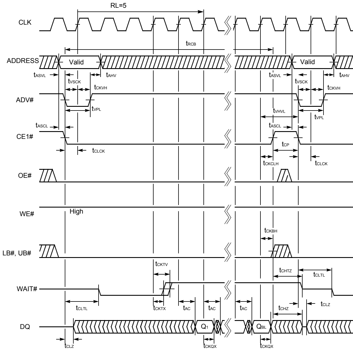
Figure II.43. 64M Synchronous Read Timing #2 (CE1# Control)
