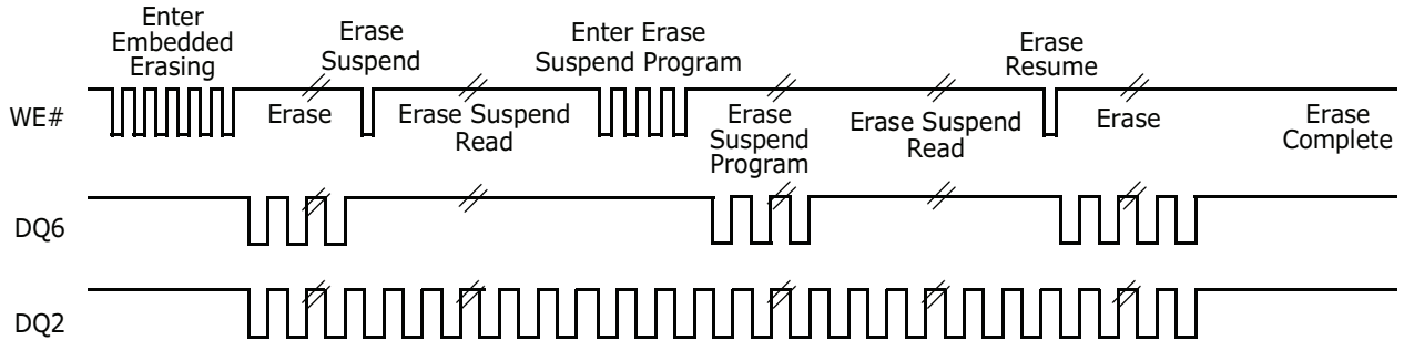
Figure 9.19. DQ2 vs. DQ6
