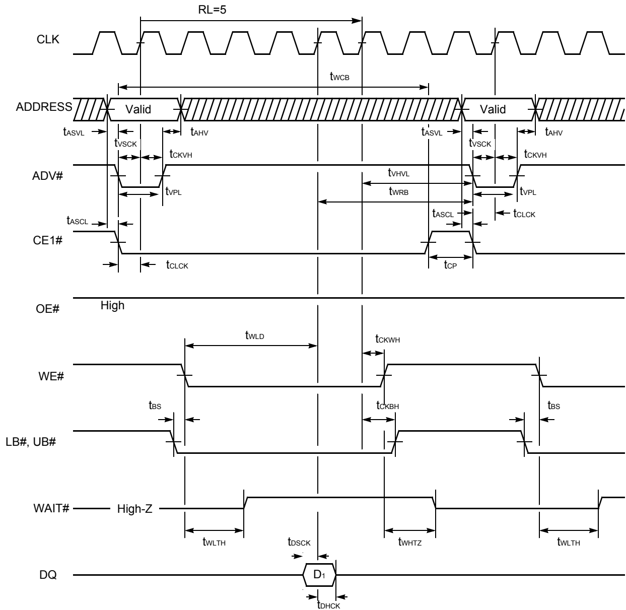
Figure II.48. Synchronous Write Timing #4 (WE# Level Control, Single Write)
