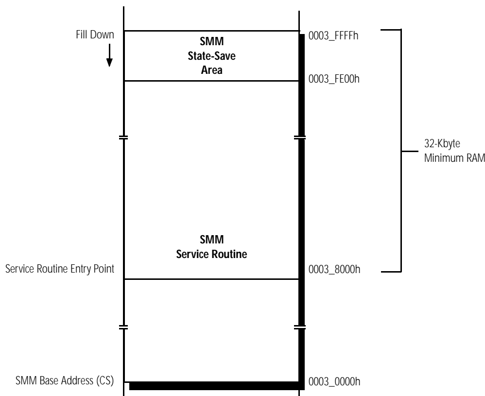
Figure 8. SMM Memory
