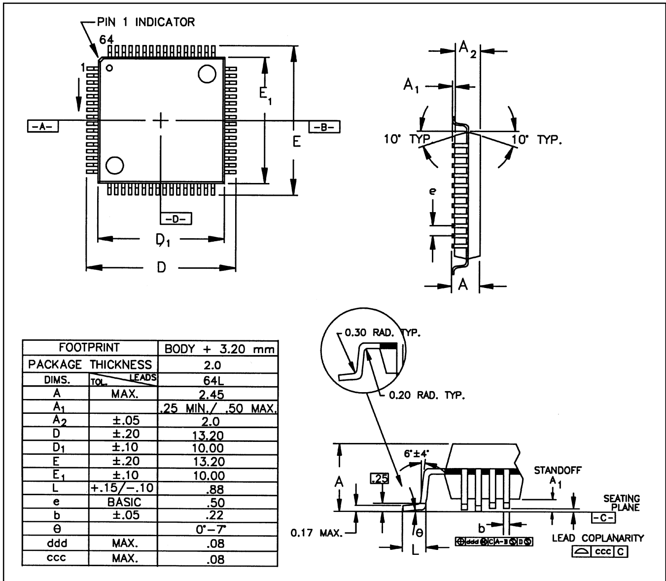
Figure 5. 64 PQFP Package
