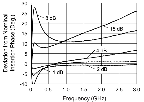
Attenuation Phase Accuracy vs. Frequency (85°C)
