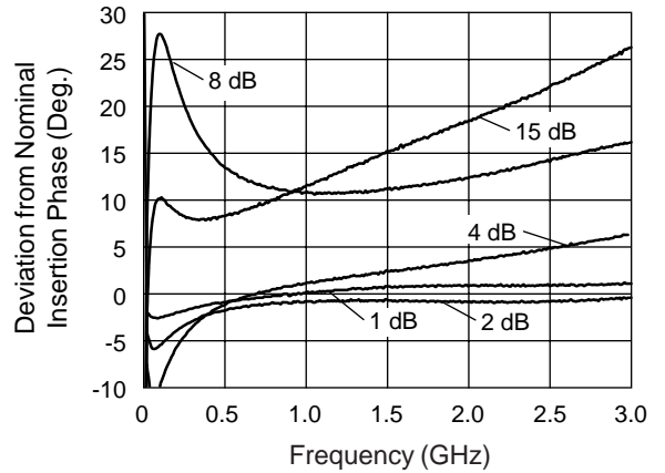
Attenuation Phase Accuracy vs. Frequency (25°C)
