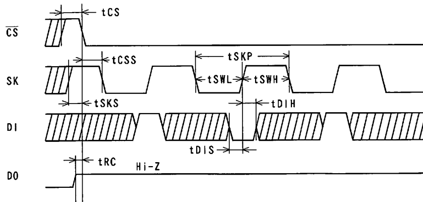
Input Waveform
