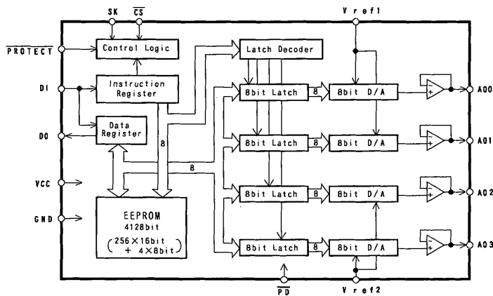
Block Diagram
