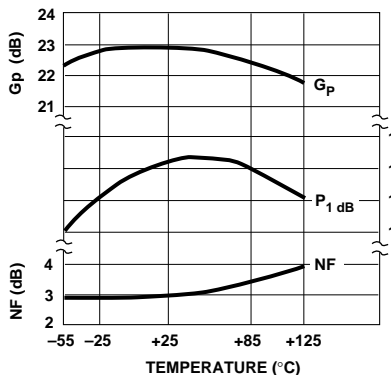
Figure 4. Output Power at 1 dB Gain Compression, NF and Power Gain vs. Case Temperature, f = 1.0 \text{ GHz} , I_d = 36 \text{ mA} .
