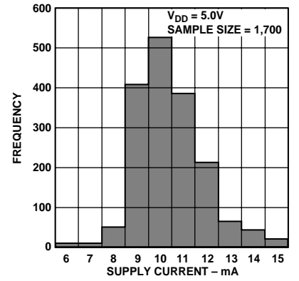
Figure 36. Supply Current Distribution
