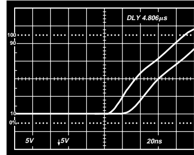
Figure 39. Saturation Recovery Time, Negative Rail
