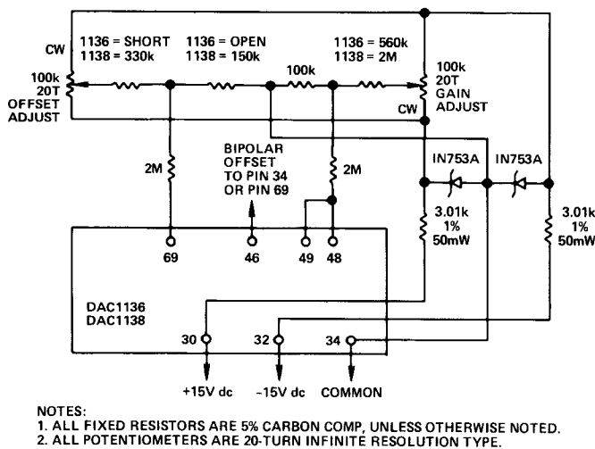
Figure 4. Gain and Offset Adjustments
