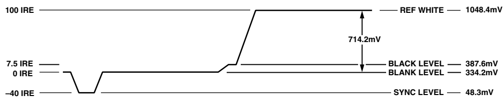
Figure 109. NTSC Luma Video Levels
