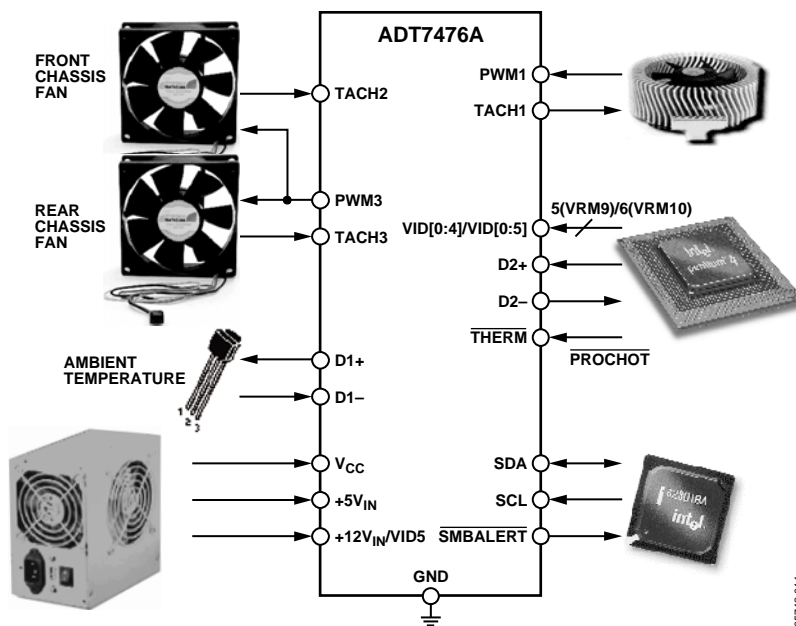
Figure 13. ADT7476A Configuration
