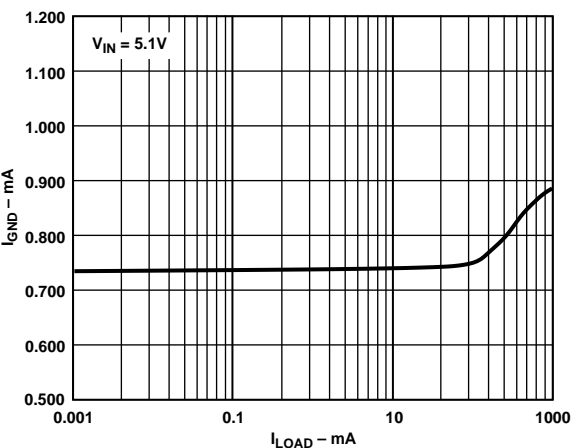
Figure 7. I_{GND} vs. I_{LOAD} ( V_{IN} = 5.1\text{ V} )*
