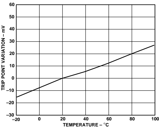
Figure 11. Variation of SU2 High Trip Point With Temperature
