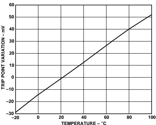
Figure 10. Variation of SU1 Low Trip Point With Temperature
