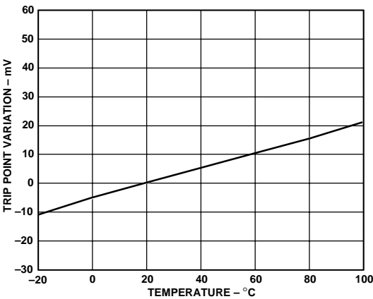
Figure 12. Variation of SU2 Low Trip Point With Temperature
