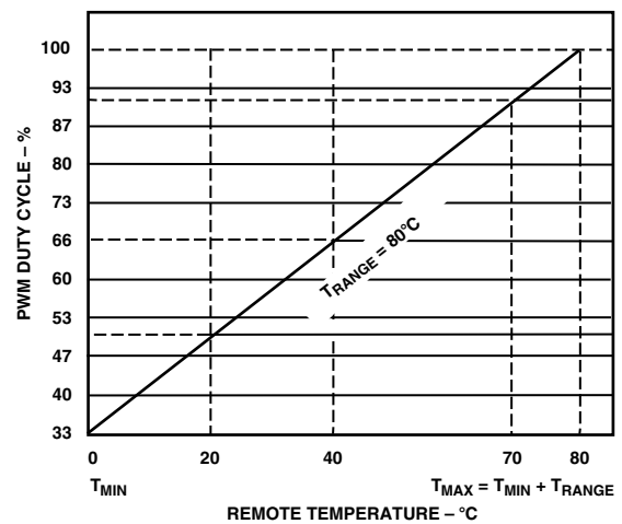
Figure 13. Max Speed Calculated by Local and Remote Temperature Control Loops Drives Fans
