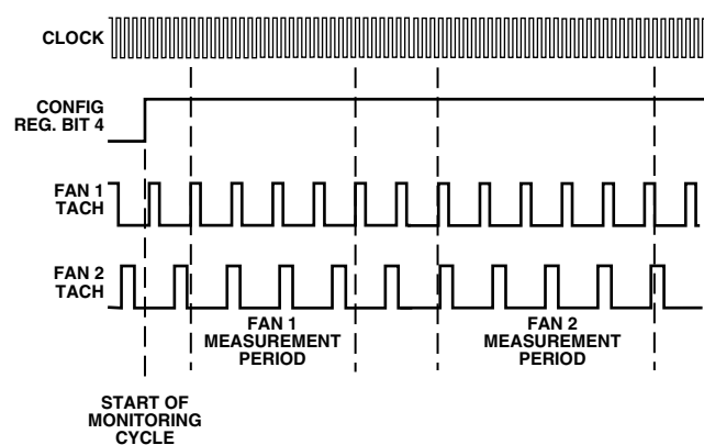
Figure 8. Fan Speed Measurement
