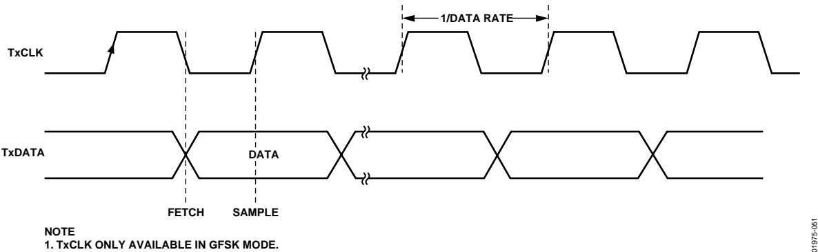
Figure 5. TxData/TxCLK Timing Diagram
