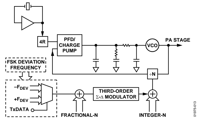
Figure 28. FSK Implementation
