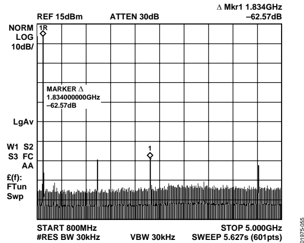
Figure 11. Harmonic Response, Murata Dielectric Filter
