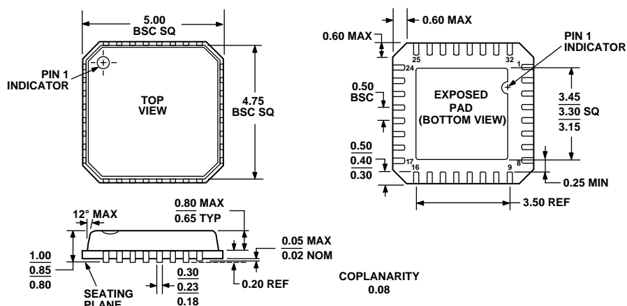
Figure 26. 32-Lead Lead Frame Chip Scale Package [VQ_LFCSP] 5 mm x 5 mm Body, Very Thin Quad (CP-32-3) Dimensions shown in millimeters
