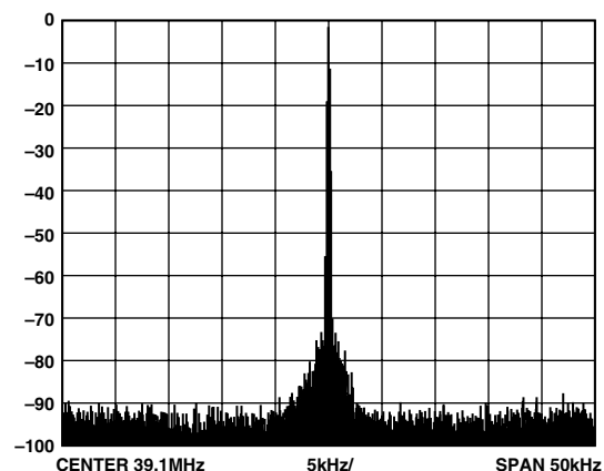
TPC 10. Narrowband SFDR, 39.1 MHz, 50 kHz BW, 30 MHz REFCLK with REFCLK Multiplier = 10×
