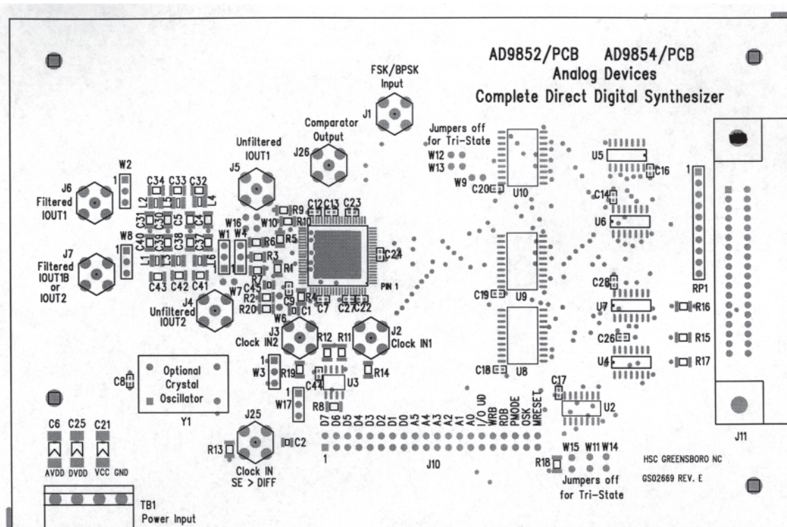
Figure 42. Assembly Drawing
