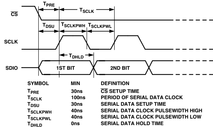
Figure 30. Timing Diagram for Data Write to AD9854
