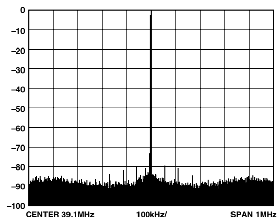
TPC 9. Narrowband SFDR, 39.1 MHz, 1 MHz BW, 30 MHz REFCLK with REFCLK Multiplier = 10×
