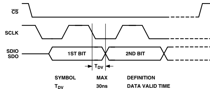
Figure 31. Timing Diagram for Read from AD9854
