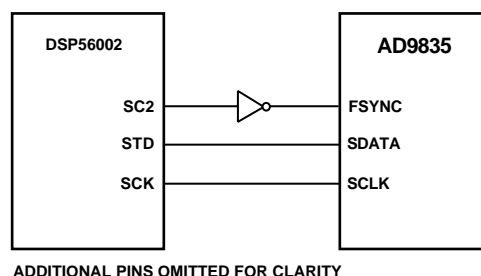
Figure 27. AD9835-to-DSP56002 Interface
