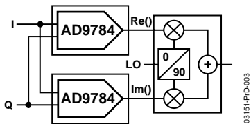
Figure 65. AD9784 Driving Quadrature Modulator
