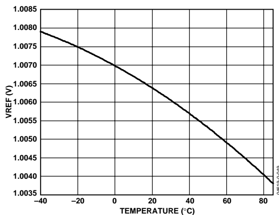
Figure 15. Typical Reference Variation with Temperature
