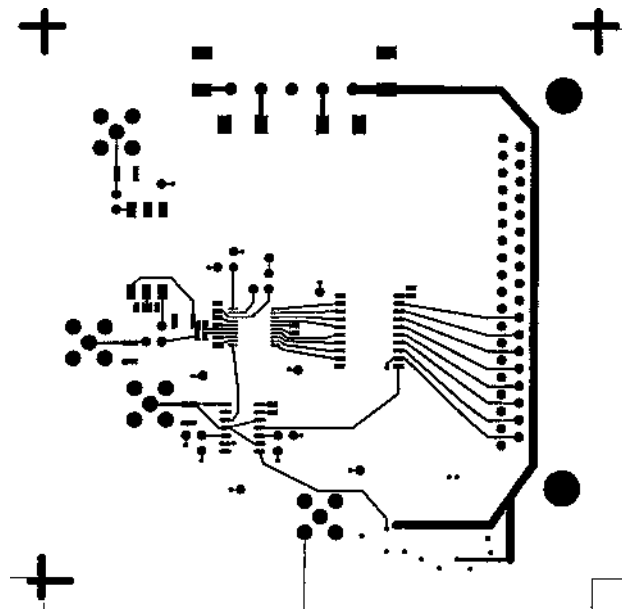
Figure 22. Printed Circuit Board Top Side Copper
