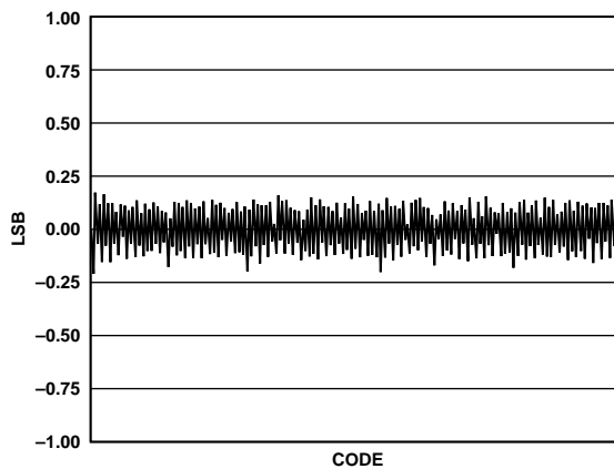
Figure 18. Differential Nonlinearity
