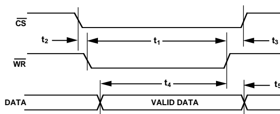
Figure 8. Write Cycle Timing
