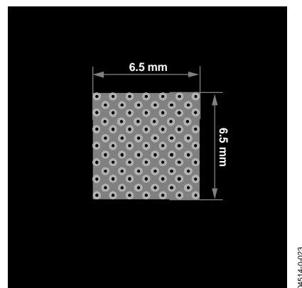
Figure 23. Land Pattern—Bottom Layer
