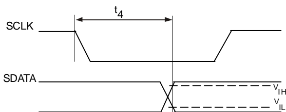
Figure 2. Access time after SCLK falling edge
