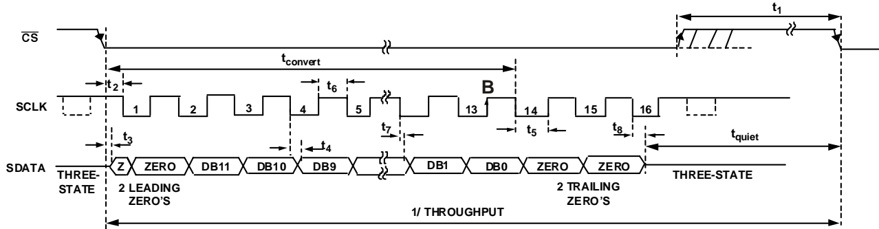
Figure 5. AD7276 Serial Interface Timing Diagram
