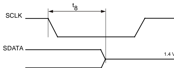
Figure 4. SCLK falling edge to SDATA Three-State
