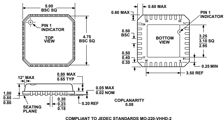
Figure 11. 32-Lead Frame Chip Scale Package [LFCSP] (CP-32) Dimensions shown in millimeters
