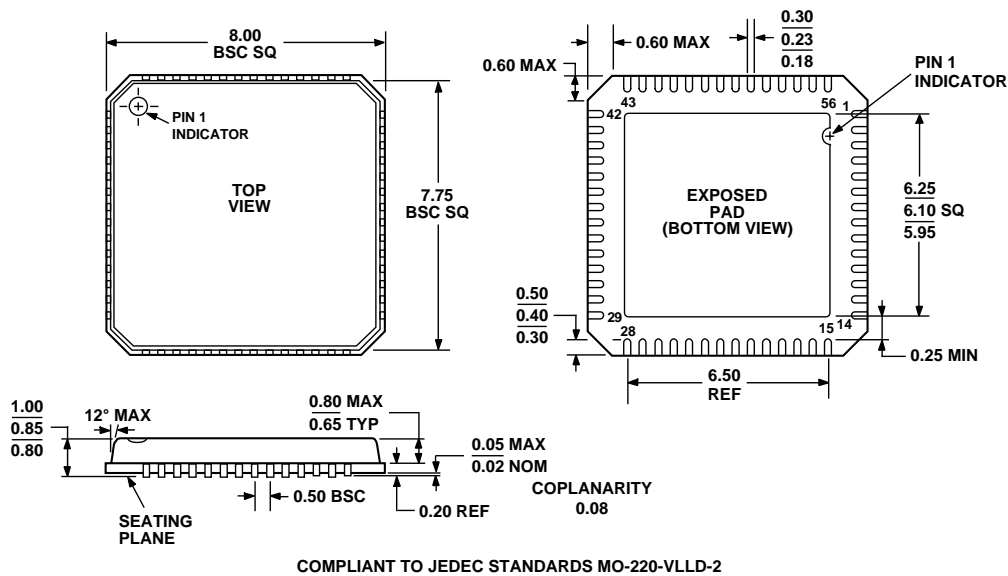
Figure 13. 56 Lead LFCSP Package Dimensions shown in millimeters
