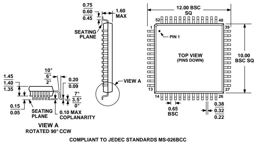
Figure 14. 52 Lead LQFP Package Dimensions shown in millimeters
